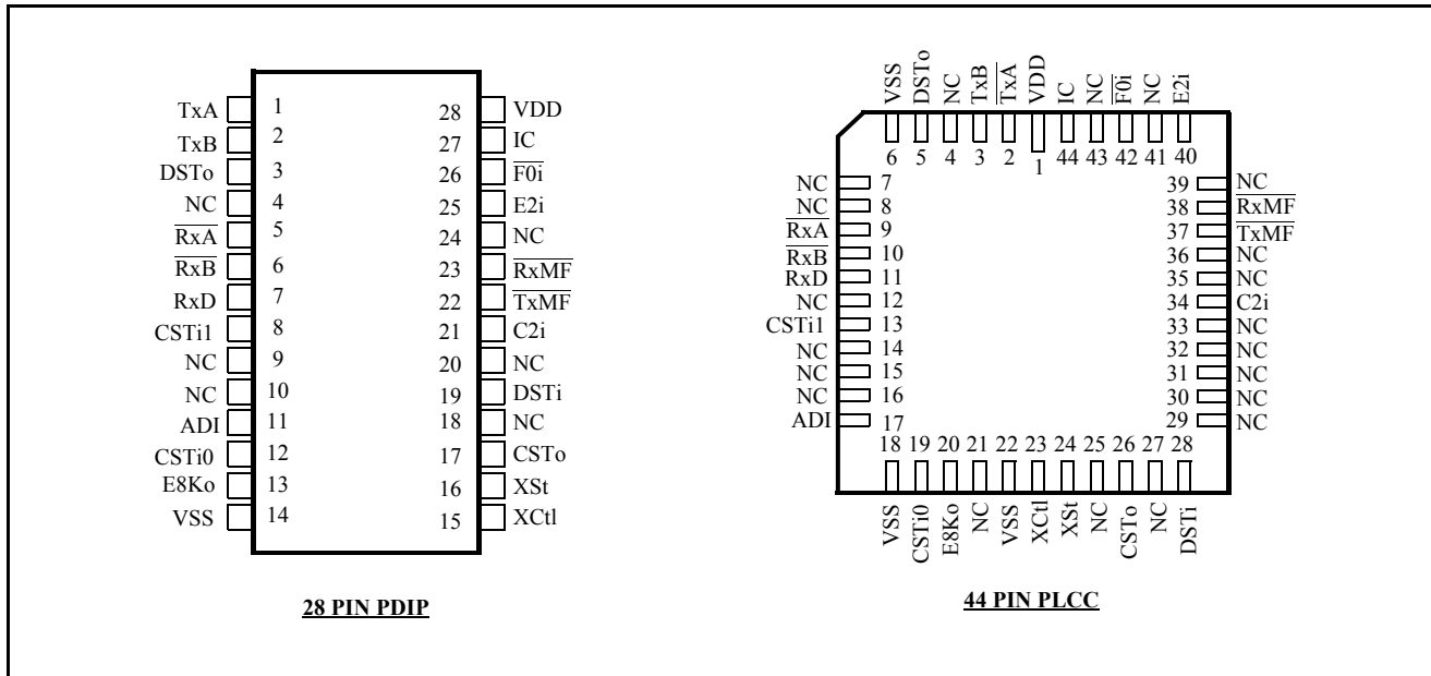
Figure 2 - Pin Connections
