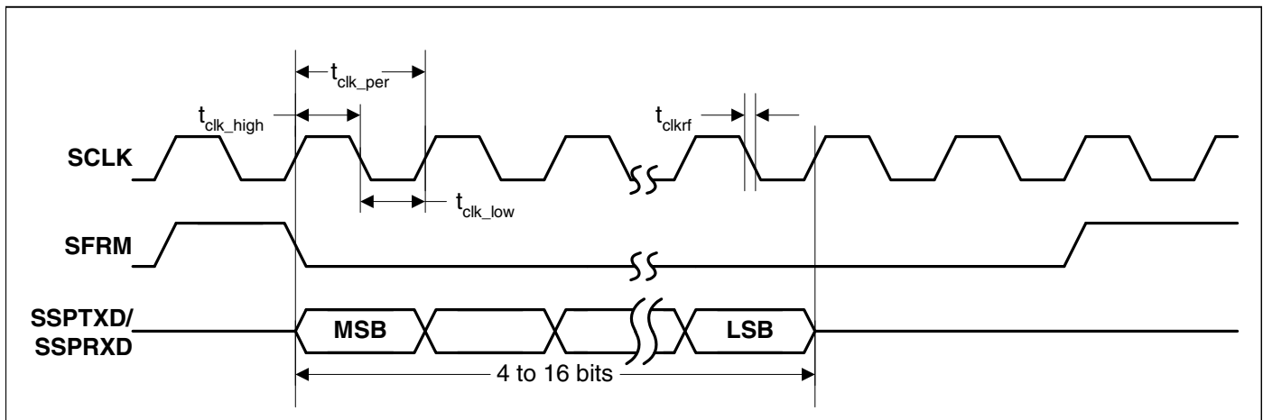
Figure 16. T / Single Transfer Timing Measurement
