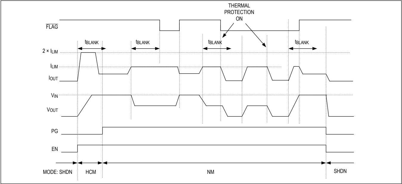
Figure 5. Continuous
