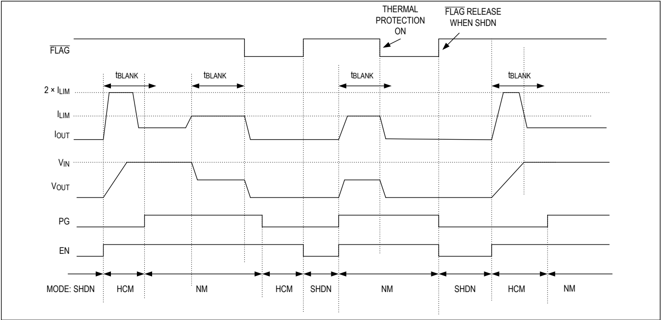
Figure 4. Latchoff
