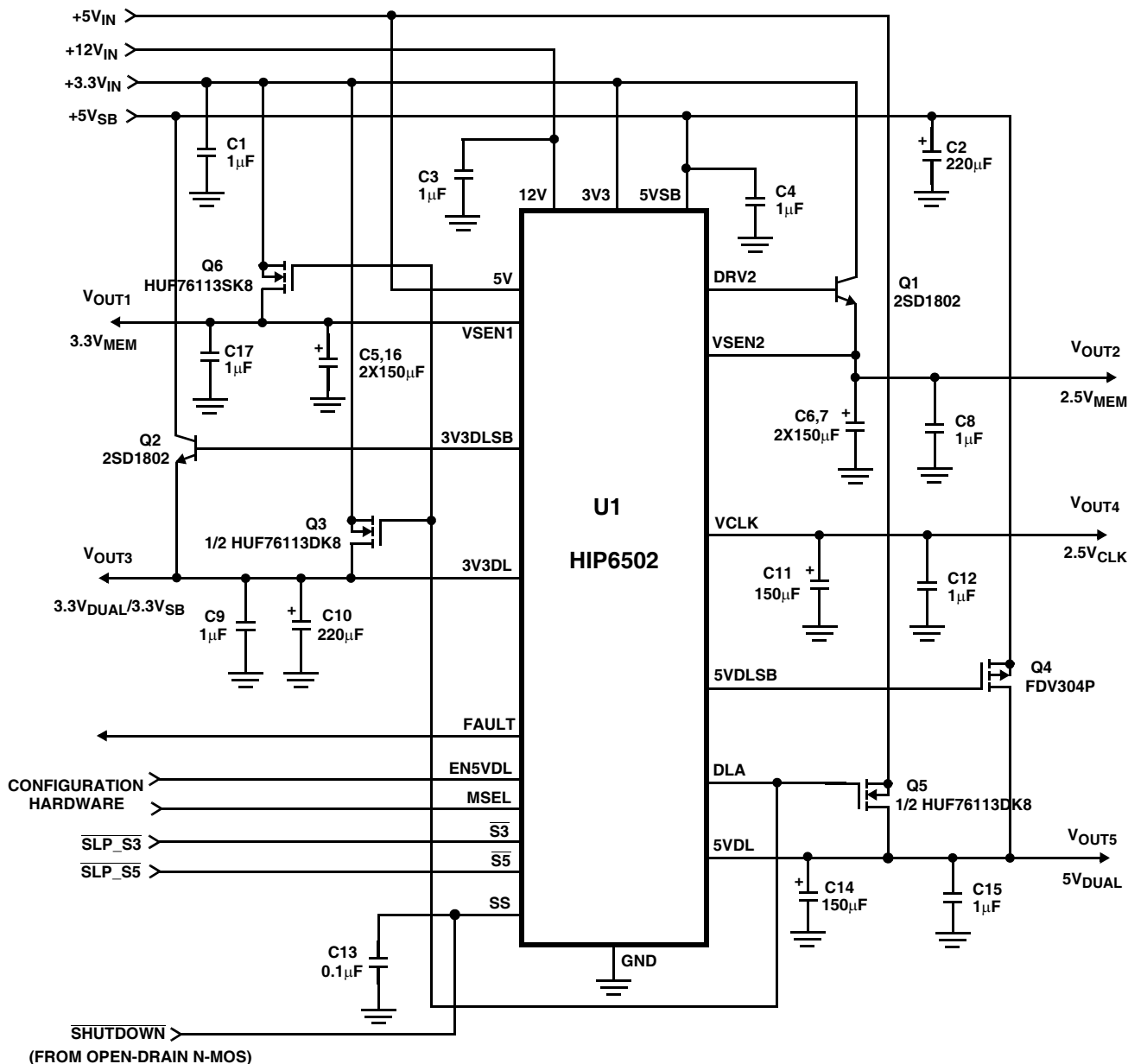
FIGURE 11. TYPICAL HIP6502 APPLICATION DIAGRAM
