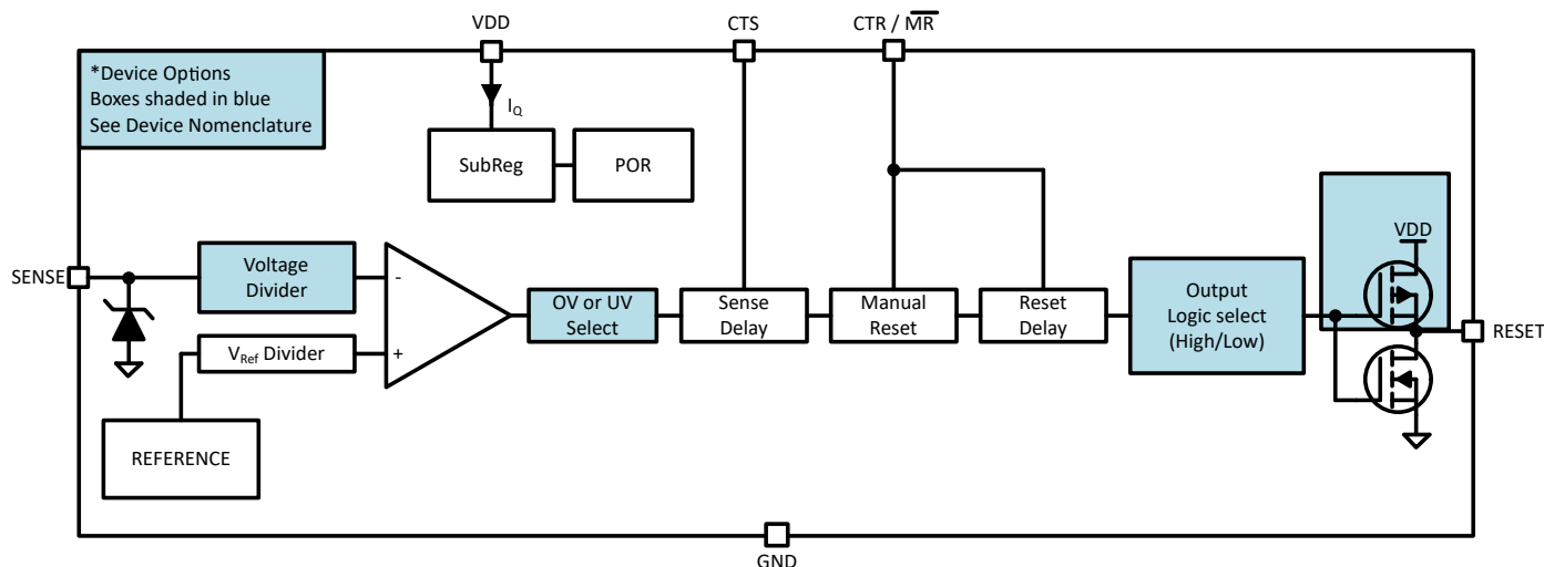
Figure 8-1. Functional Block Diagram 1
