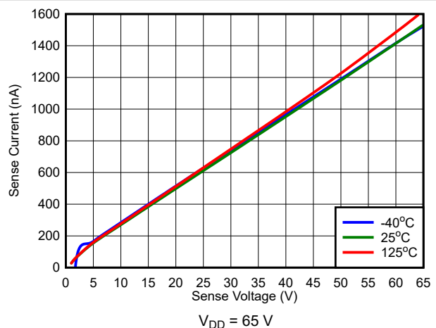
Figure 7-8. V_{SENSE} vs I_{SENSE}
