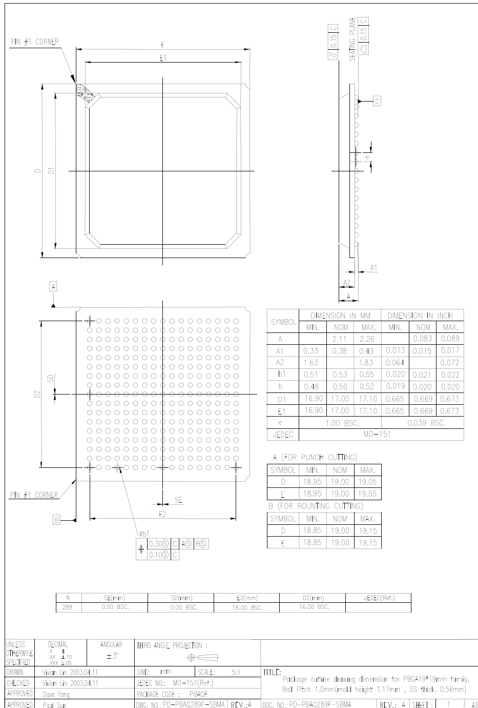
289-Pin PBGA
