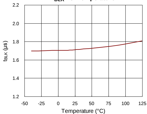
t_{BLK} vs. Temperature
