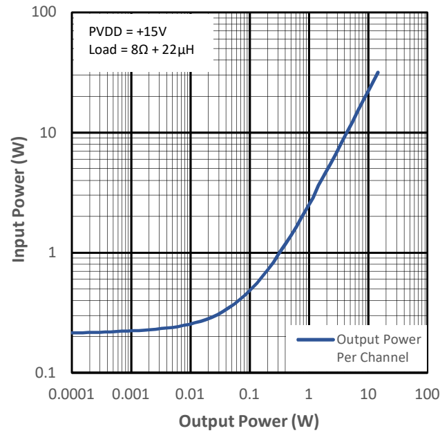
Figure 13-16 Input Power vs Output Power for PMP4
