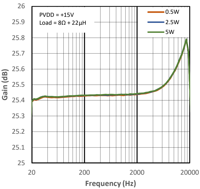
Figure 13-22 Gain vs Frequency for PMP1
