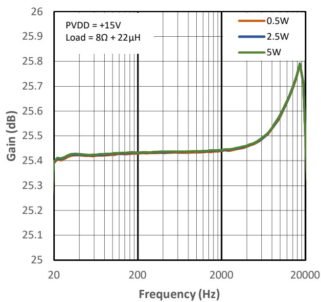
Figure 13-23 Gain vs Frequency for PMP2
