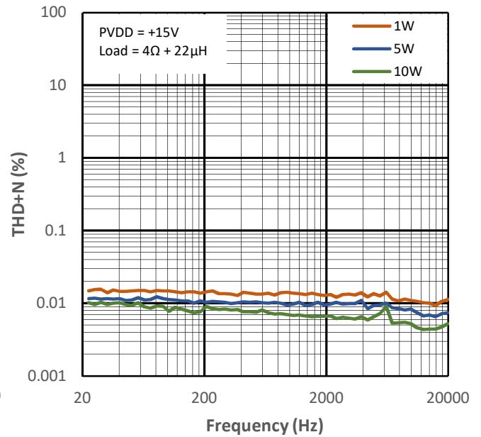
Figure 12-6 THD+N vs Frequency for PMP1
