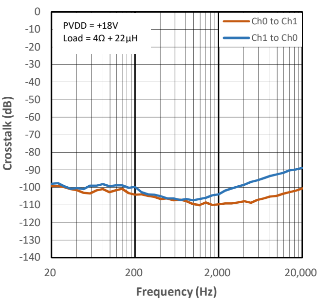
Figure 10-30 Crosstalk vs Frequency for PMP1
