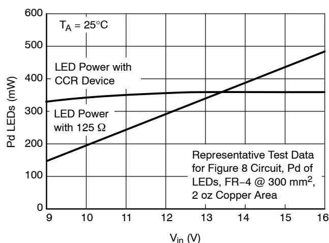
Figure 11. LED Power
