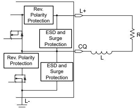
Figure 9-3. N-Switch Mode
