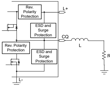
Figure 9-2. P-Switch Mode
