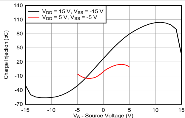
Figure 6-14. Charge Injection vs Source Voltage – Dual Supply
