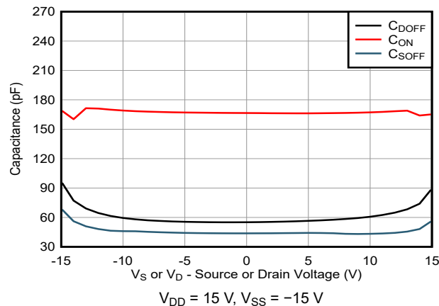
Figure 6-25. Capacitance vs Source or Drain Voltage
