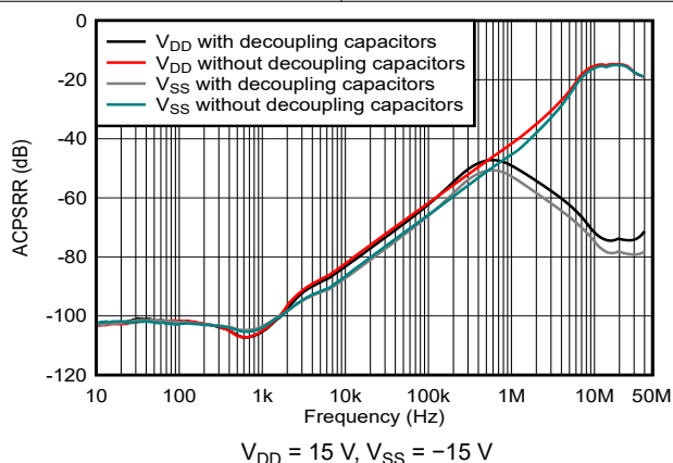
Figure 6-29. ACPSRR vs Frequency
