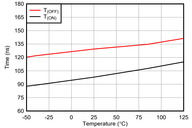
Figure 6-20. T_{\text{ON (EN)}} and T_{\text{OFF (EN)}} vs Temperature
