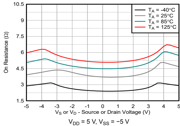
Figure 6-7. On-Resistance vs Temperature
