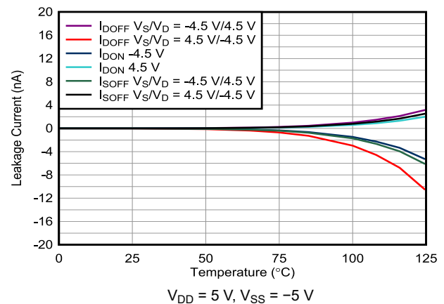
Figure 6-12. On-Leakage vs Temperature
