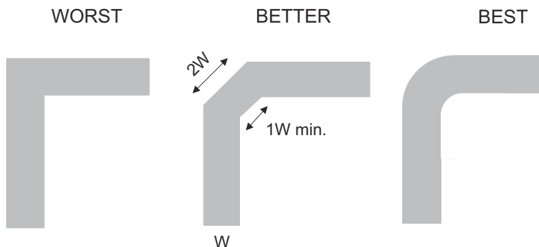
Figure 11-1. Trace Example
