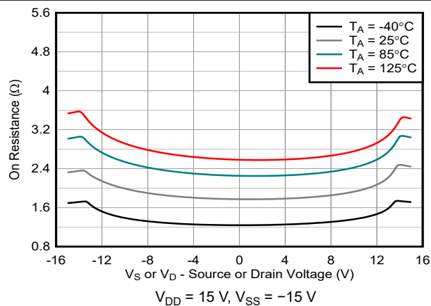
Figure 6-5. On-Resistance vs Temperature
