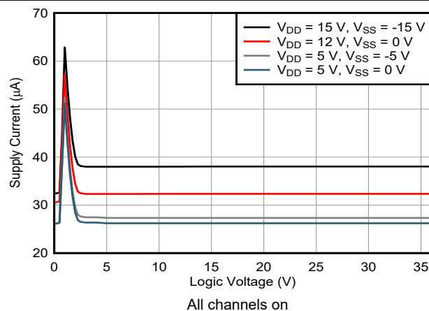
Figure 6-13. Supply Current vs Logic Voltage
