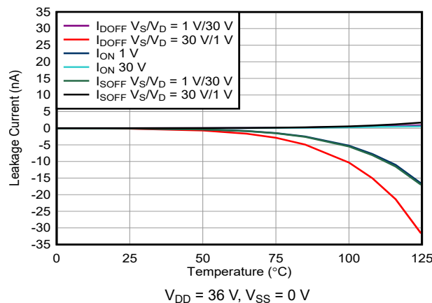
Figure 6-11. On-Leakage vs Temperature
