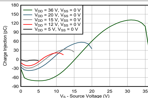
Figure 6-16. Charge Injection vs Source Voltage – Single Supply
