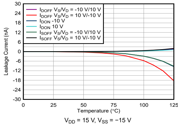
Figure 6-9. On-Leakage vs Temperature
