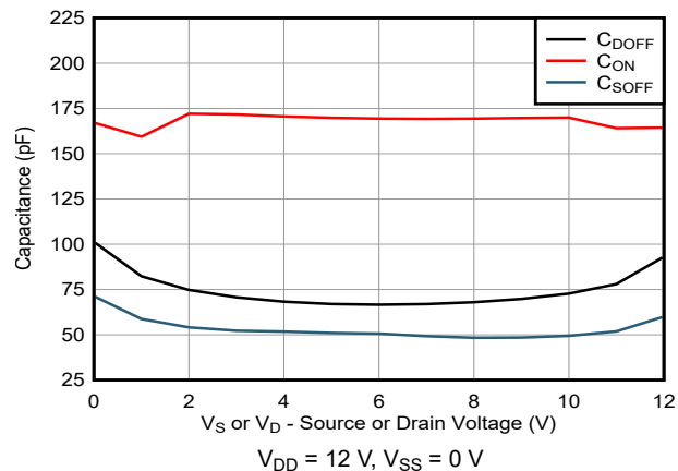
Figure 6-26. Capacitance vs Source or Drain Voltage
