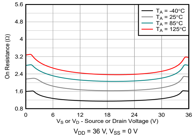
Figure 6-8. On-Resistance vs Temperature
