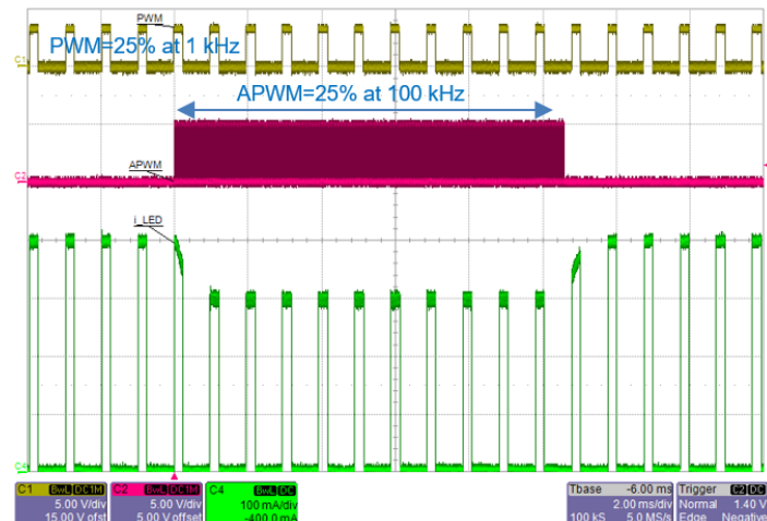
Figure 32: PWM = 25% at 1 kHz. Peak LED current drops from 400 mA ( 4 \times 100 \text{ mA/ch} ) to 300 mA when APWM of 25% duty cycle is applied
