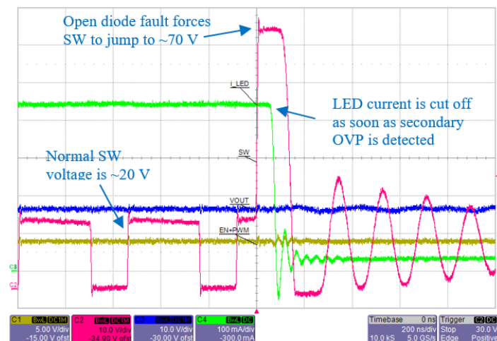
Figure 42: An open-diode fault is introduced during normal operation. SW voltage jumps to ~70 V, causing the MOSFET to self-conduct and dissipate energy in the inductor.
