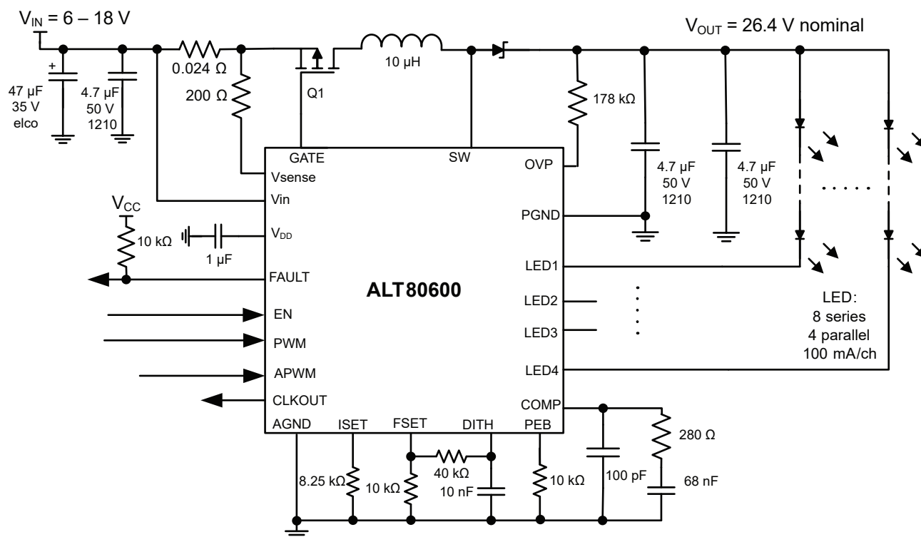
Figure 49: ALT80600 Design Example Schematic
