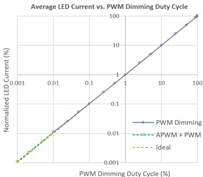
Figure 33: How to achieve 100,000:1 dimming ratio by using both PWM and APWM. Test conditions: V_{IN} = 12\text{ V} , V_{OUT} = 25\text{ V} ( 8 \times \text{WLED} ), total LED current = 400 mA, PWM frequency = 200 Hz, APWM frequency = 100 kHz.
