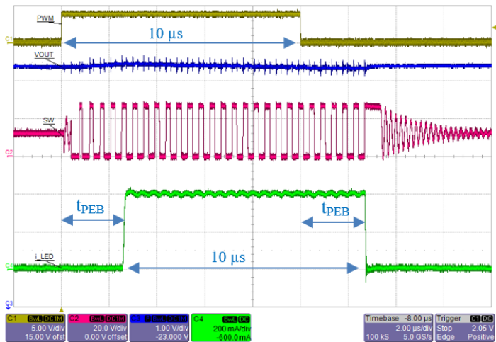
Figure 21: Zoom in view for PWM on-time = 10 μs. Notice that the LED current is shifted with respect to PWM signal. Ripple at V OUT
