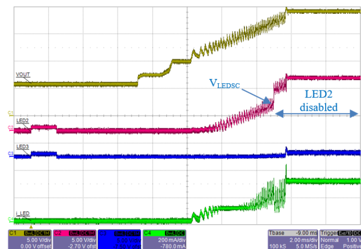
Figure 40: Startup sequence when LED string#2 has a partial-short fault (4 x WLED instead of 6). As soon as LED2 pin rises above V_{LEDSC} (~4.6 V), the channel is disabled. Output is now 300 mA.
