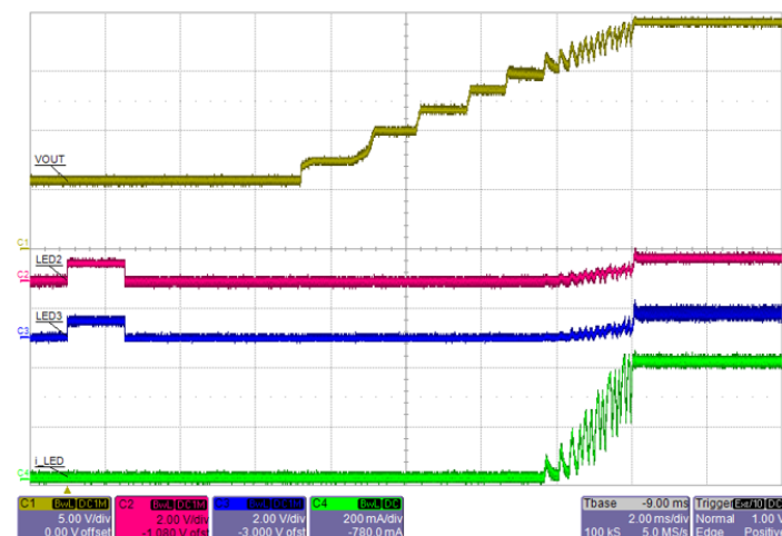
Figure 39: Normal startup sequence showing voltage at LED2 and LED3 pins. V_{IN} = 6 V, output = 6 x WLED in series, current = 4 x 100 mA
