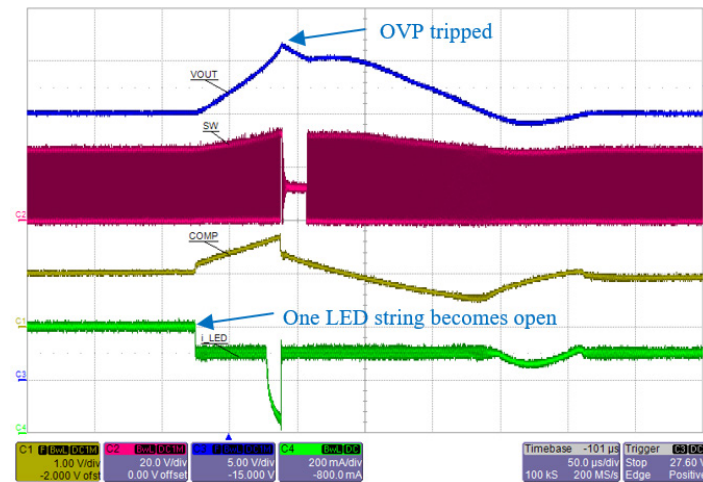
Figure 41: An open-LED string faults causes V_{OUT} to ramp up and trip OVP. The ALT80600 then disables the open LED string and continues with remaining strings.
