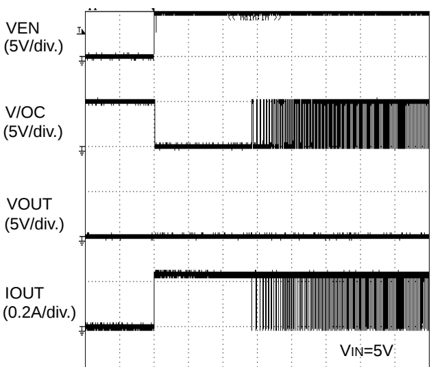
Figure 37. Over-current response enable to shortcircuit
