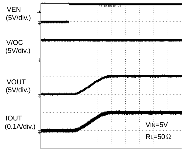
TIME (1ms/div.) Figure 32. Output rise characteristic
