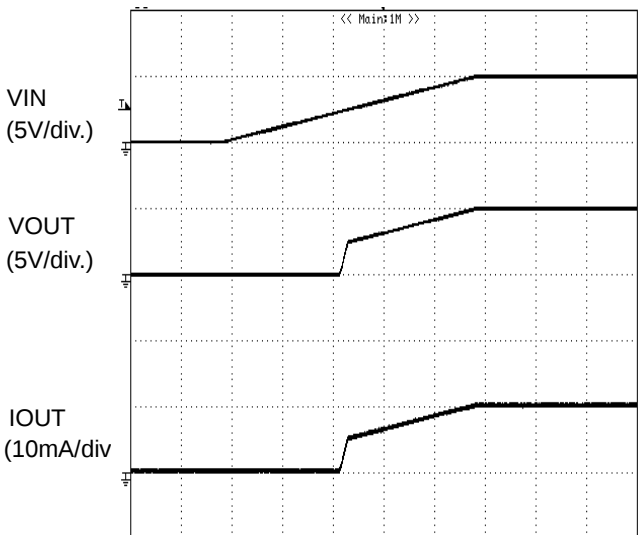
Figure 39. UVLO response increasing VIN
