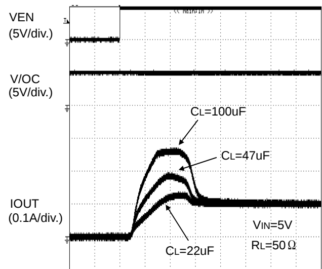
TIME (1ms/div.) Figure 34. Inrush current response
