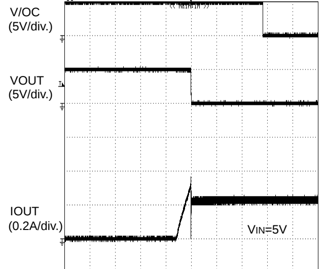
TIME (5ms/div.) Figure 35. Over-current response ramped load
