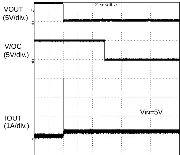
Figure 38. Over-current response 1Ω load to enabled device
