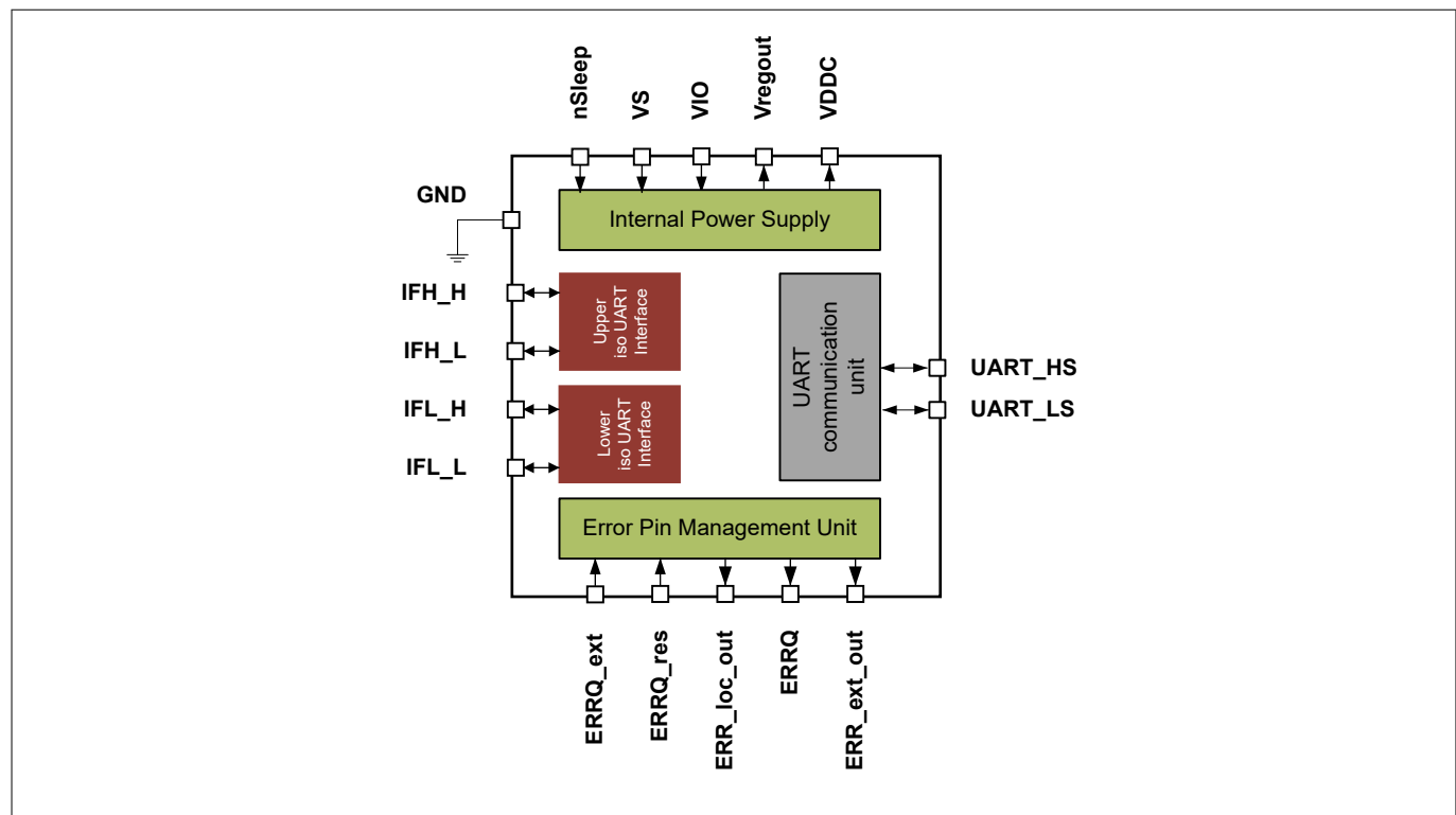
Figure 1 Block diagram
