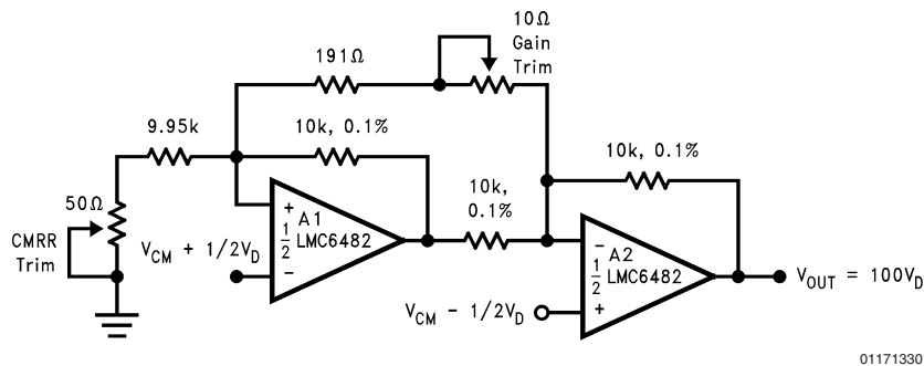
FIGURE 16. Low-Power Two-Op-Amp Instrumentation Amplifier
