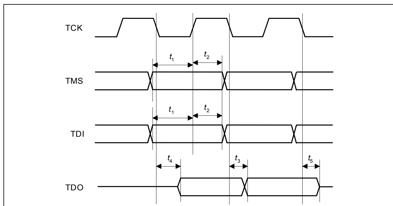
Figure 43 JTAG Timing
