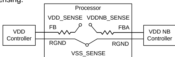
Figure 5. Differential Remote Voltage Sense Connection
