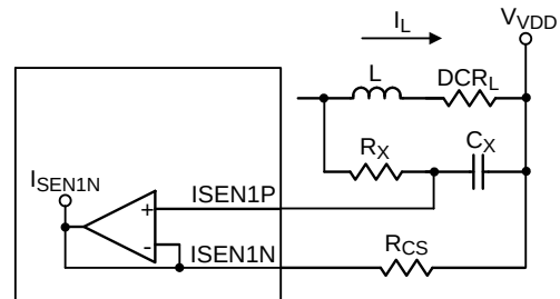
Figure 12. VDD Controller : Lossless Inductor Sensing
