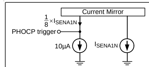
Figure 20. VDDNB Controller : Per-Phase OCP Setting
