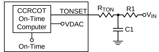
Figure 11. VDD Controller : On-Time Setting with RC Filter
