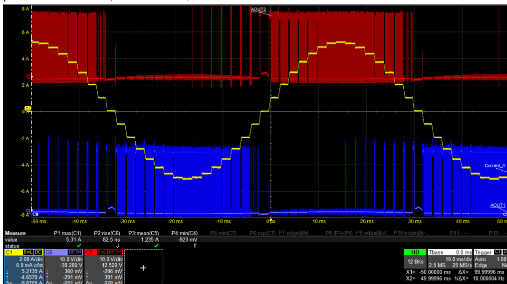
Figure 7-11. Current regulation with internal reference voltage
