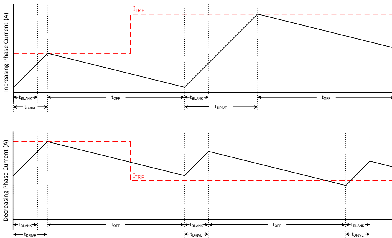
Figure 7-13. Slow Decay Mode
