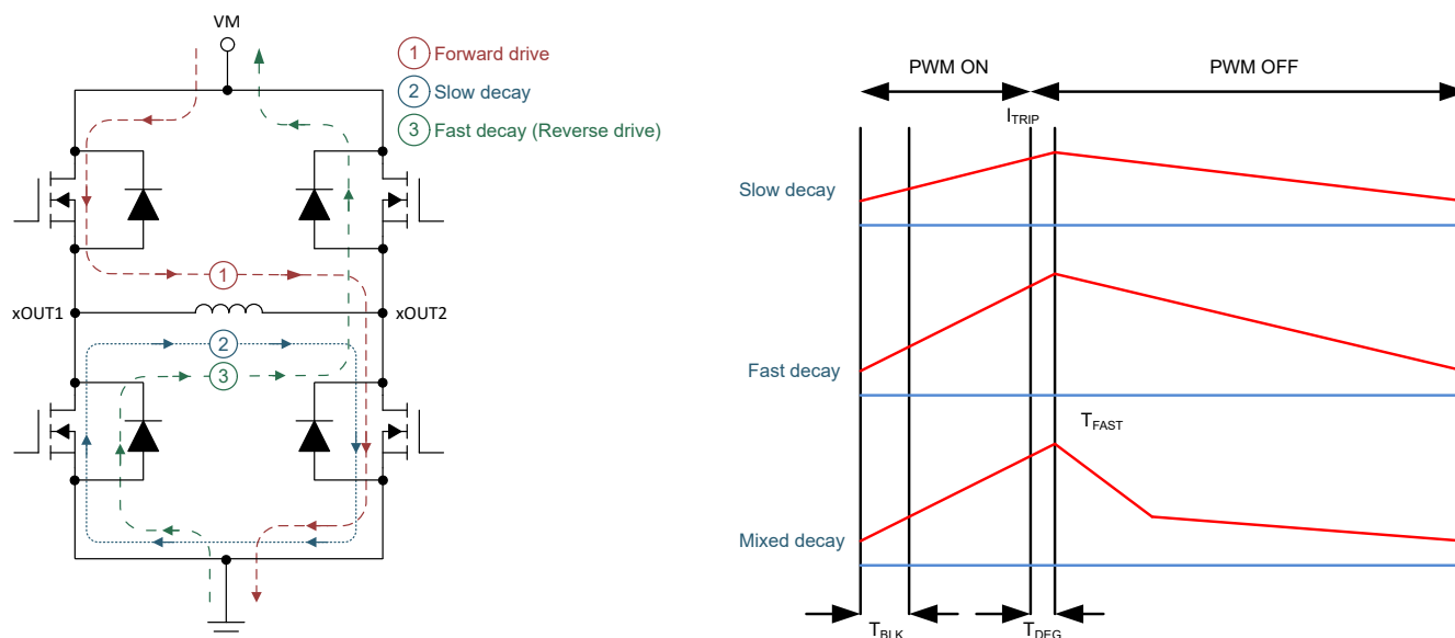
Figure 7-12. Decay Modes
