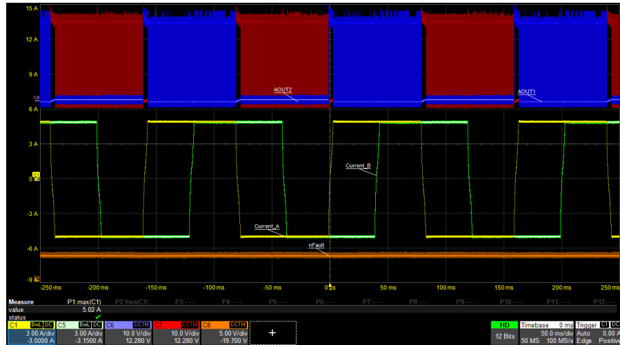
Figure 8-3. Full-step at 25 pps with I_{FS} = 5 A
