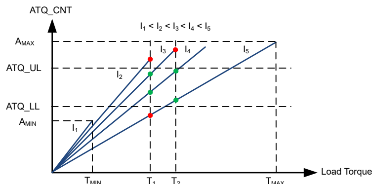
Figure 7-27. ATQ_CNT as a function of load torque
