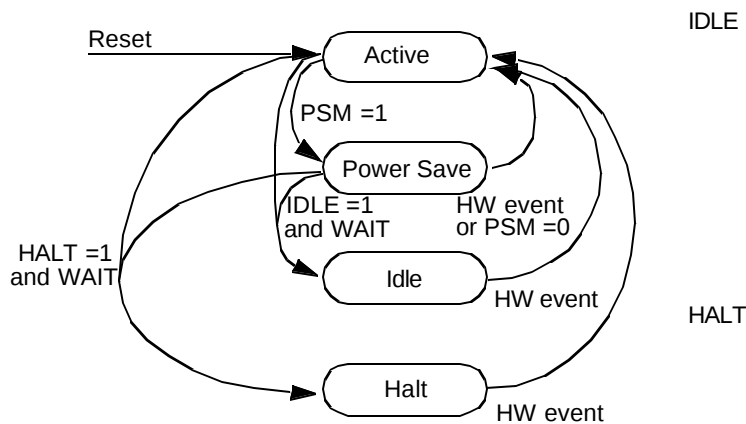
Figure 6. Power Modes and Transitions
