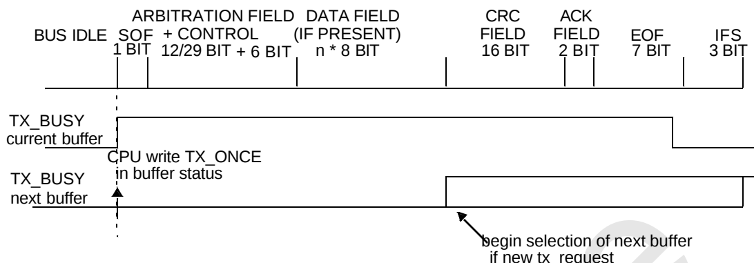
Figure 64. Data Transmission
