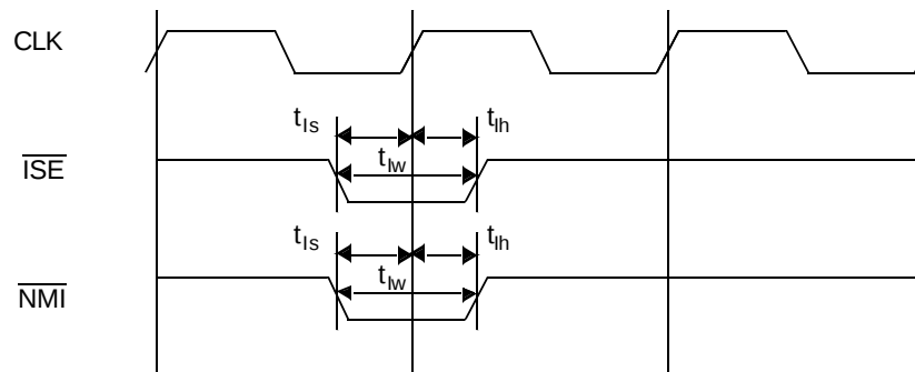
Figure 78. ISE & NMI Signal Timing
