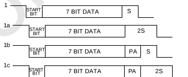
Figure 35. Seven Data Bit Frame Options
