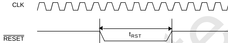
Figure 79. Non-Power-On Reset
