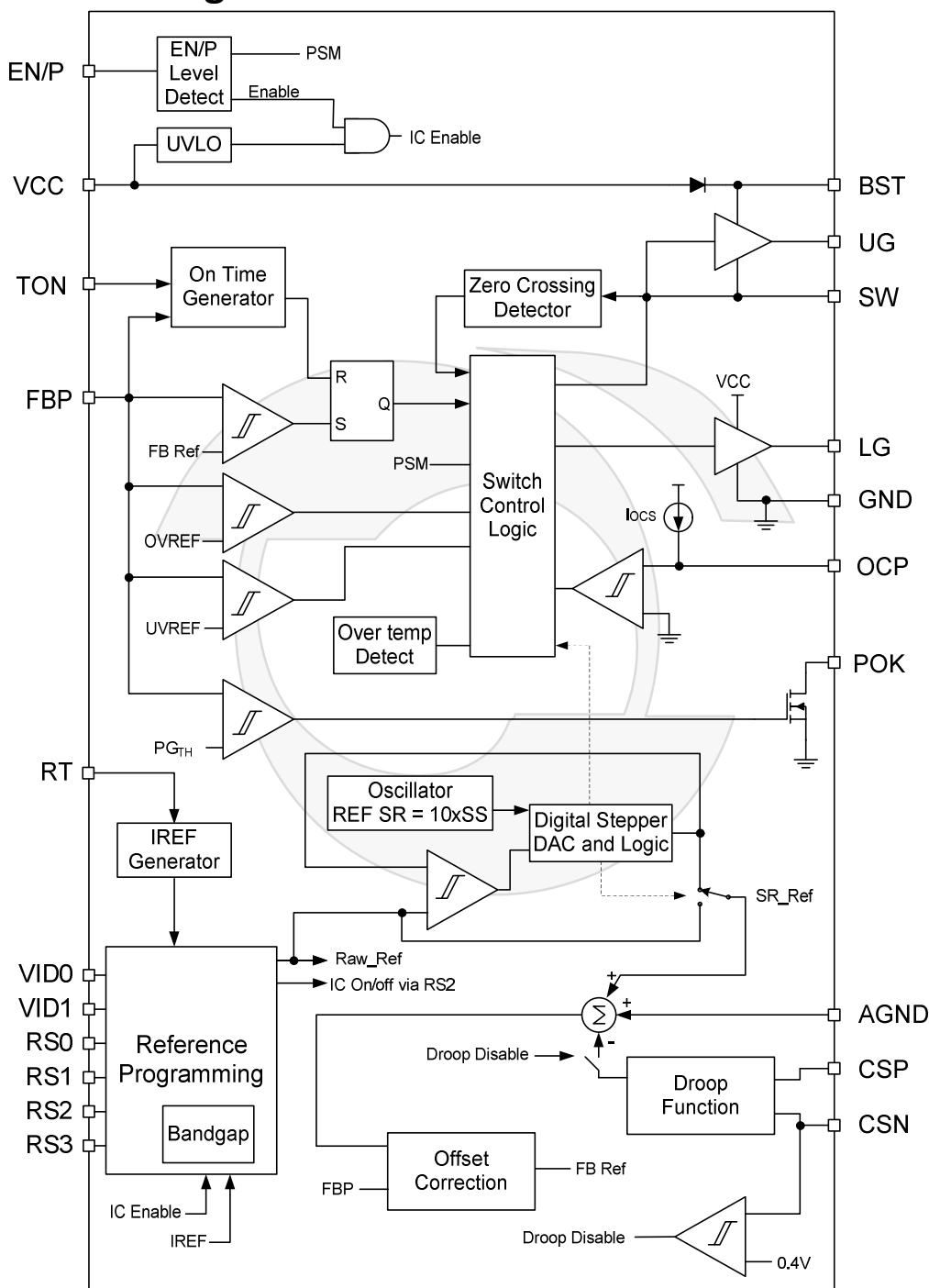
Figure 4: Block Diagram
