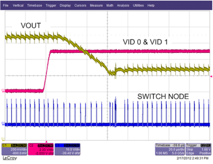
Figure 14. VID Change – High to Low
