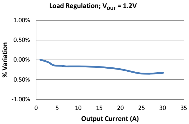
Figure 10. Load Regulation
