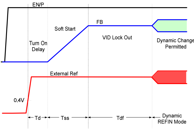
Figure 7. REFIN Power On Timing – Case 2
