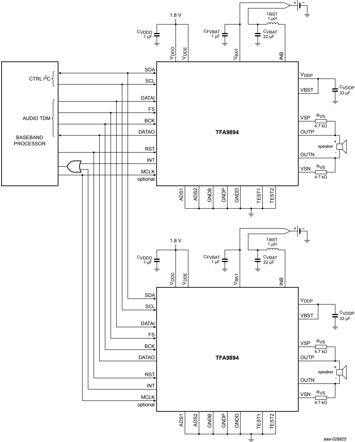
Figure 7. Typical stereo application
