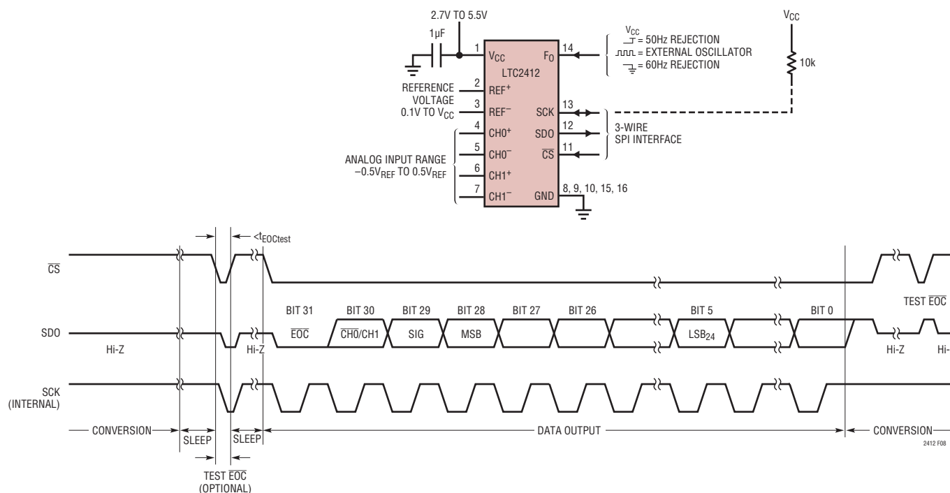
Figure 8. Internal Serial Clock, Single Cycle Operation
