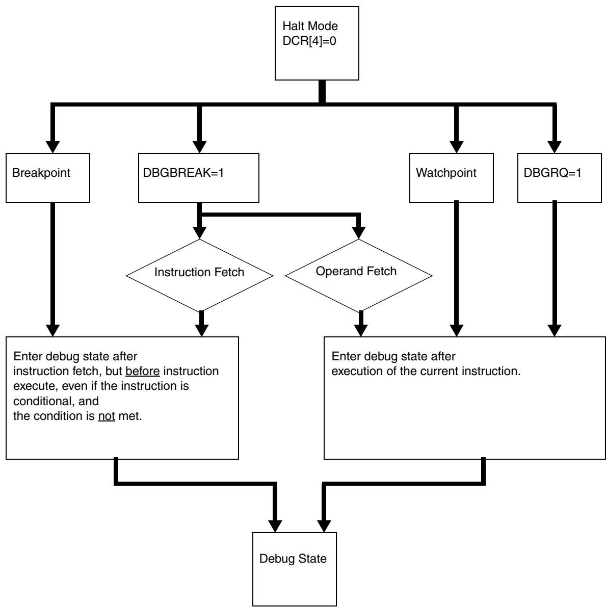
Figure 8-9. Halt Mode Overview
