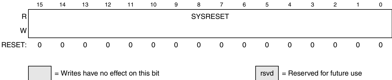
Figure 25-6. System Reset (SYSRESET) Register
