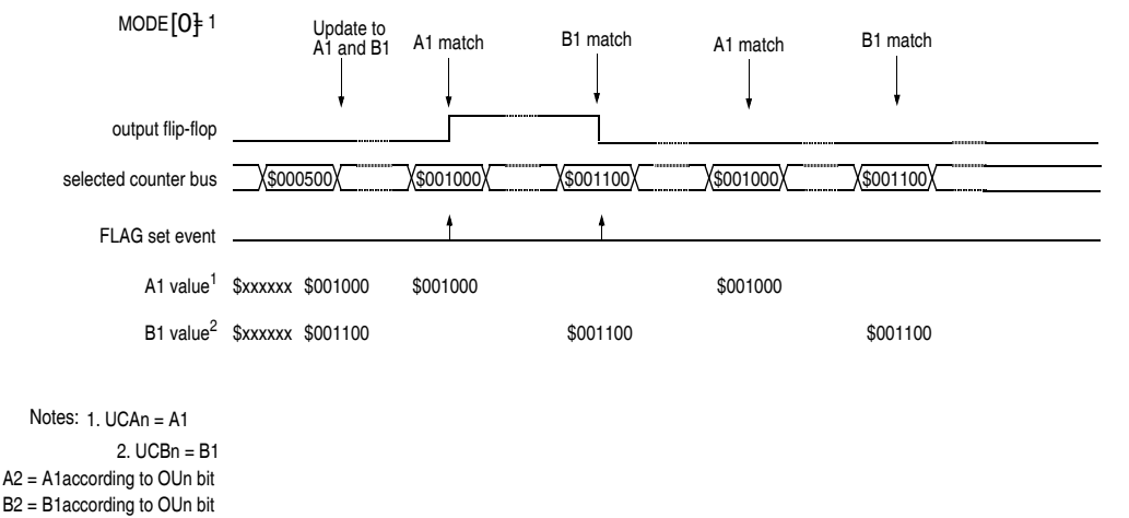
Figure 32-22. Double Action Output Compare with FLAG set on both matches
