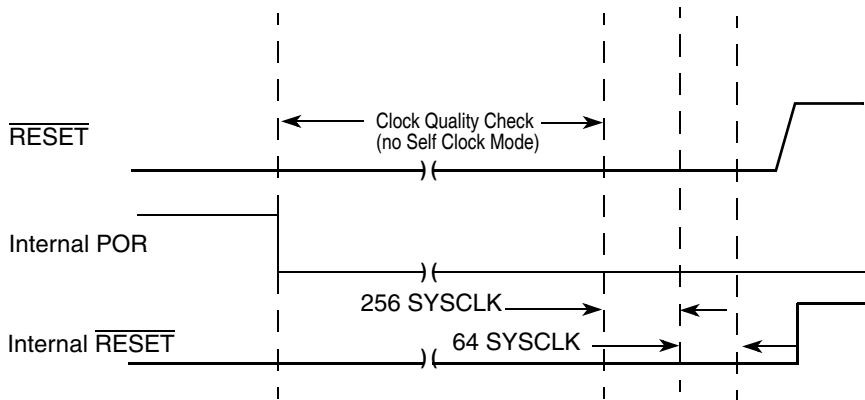
Figure 23-21. \overline{\text{RESET}} Pin Held Low Externally
