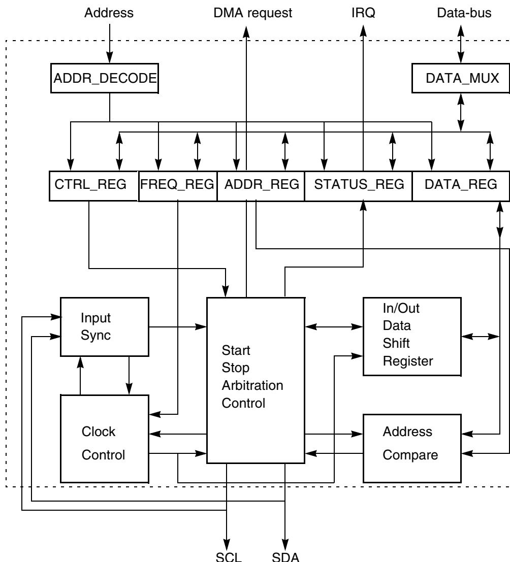
Figure 29-2. I²C Module DMA Interface Block Diagram
