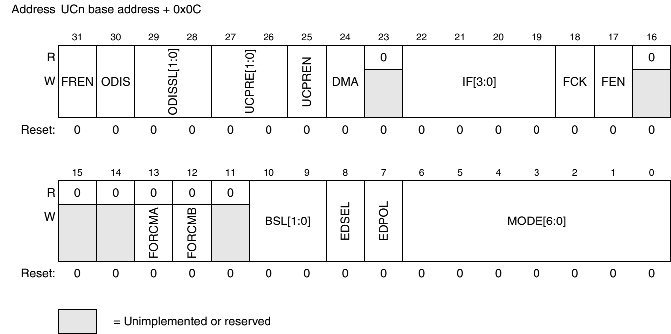
Figure 32-10. eMIOS Control Register (UCCRn)
