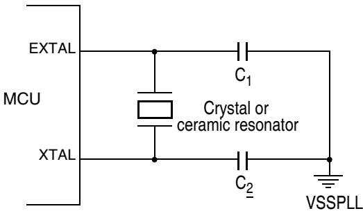
Figure 24-2. ALC Oscillator Connections ( \overline{XCLKS}=1 )
