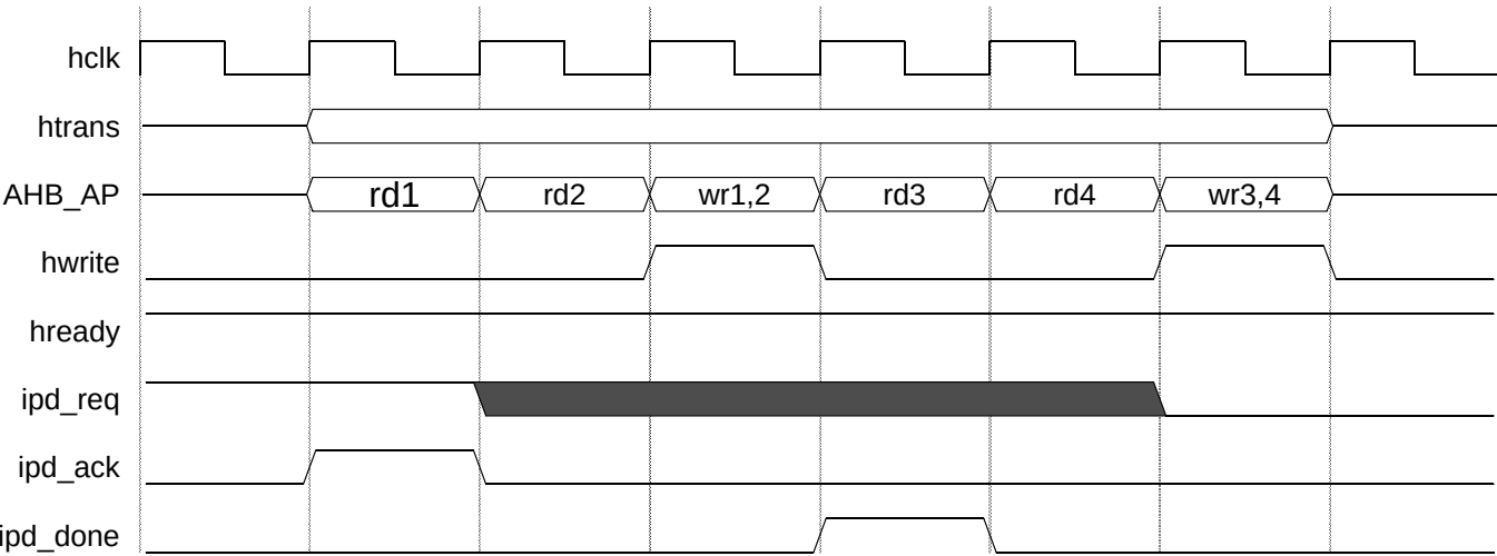
Figure 12-25. ipd_req removal
