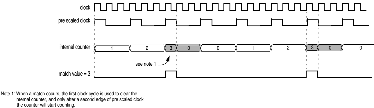
Figure 32-58. Time base period when running with a pre scaler ratio greater than 1
