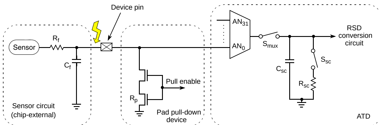
Figure 33-21. Predischarge Circuit
