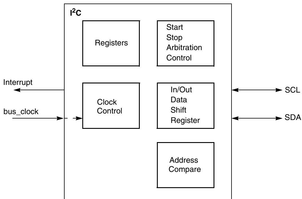
Figure 29-1. I²C Block Diagram
