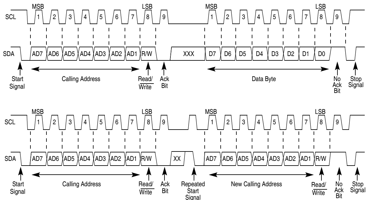
Figure 29-12. I²C Bus Transmission Signals
