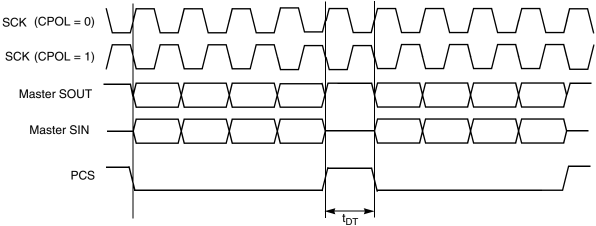
Figure 30-22. Continuous SCK Timing Diagram (CONT=0)
