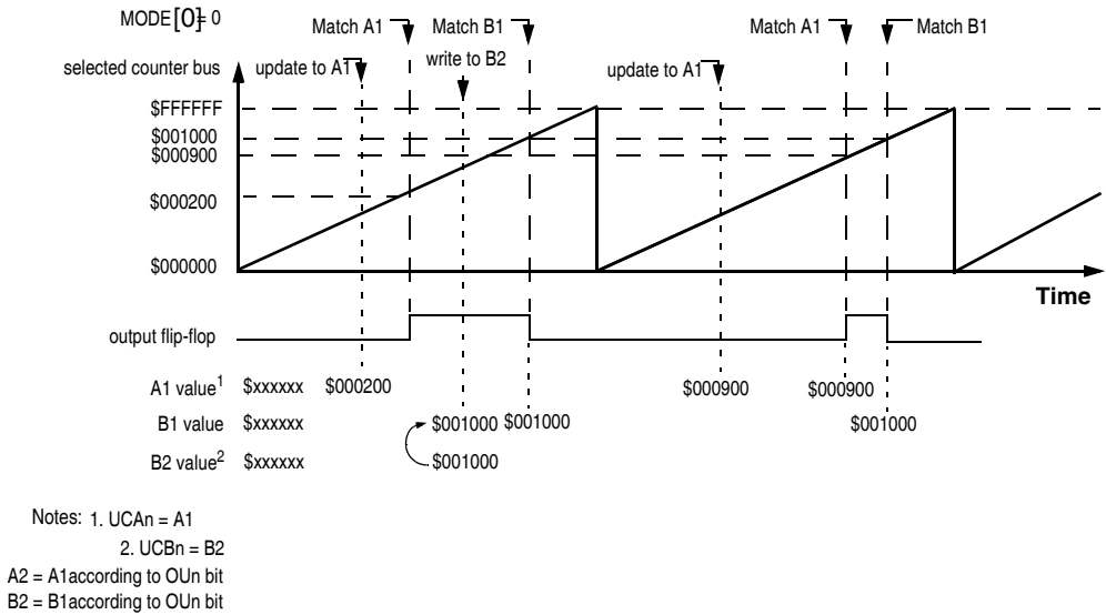
Figure 32-49. Output PWM with immediate update
