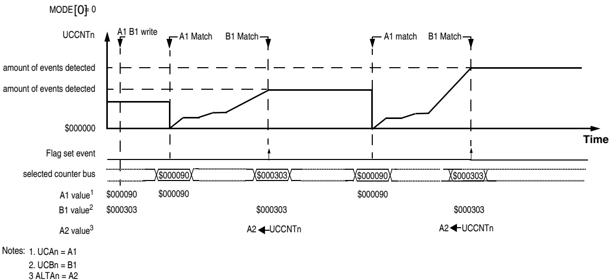
Figure 32-25. Pulse/Edge Counting continuous mode example
