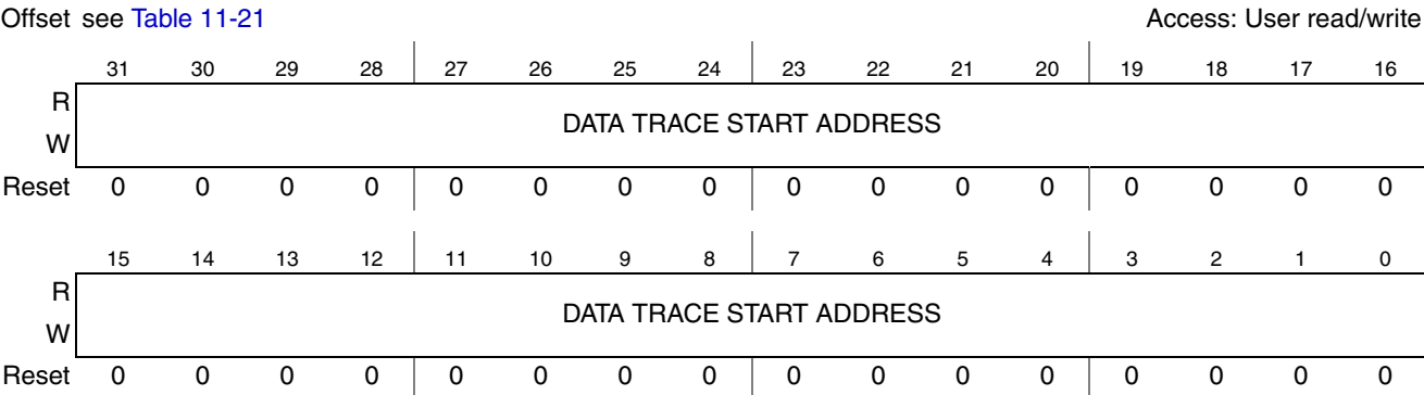
Figure 11-14. Data Trace Start Address Registers (DTSA1, DTSA2)
