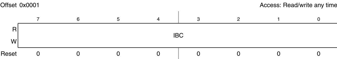
Figure 29-5. I 2 C Bus Frequency Divider Register (IBFD)
