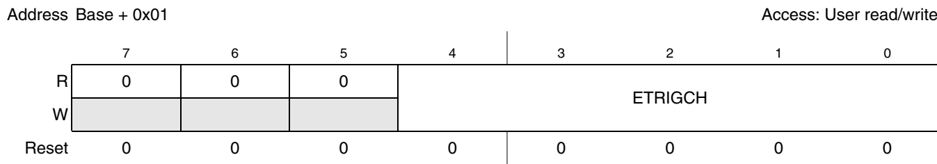
Figure 33-3. ATD External Trigger Channel Register (ATDETRIGCH)
