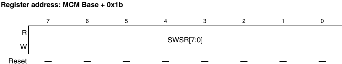
Figure 13-9. Miscellaneous Software Watchdog Timer Service (MSWTSR) Register
