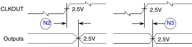
Figure A-3. General Purpose Output Timing Specifications
