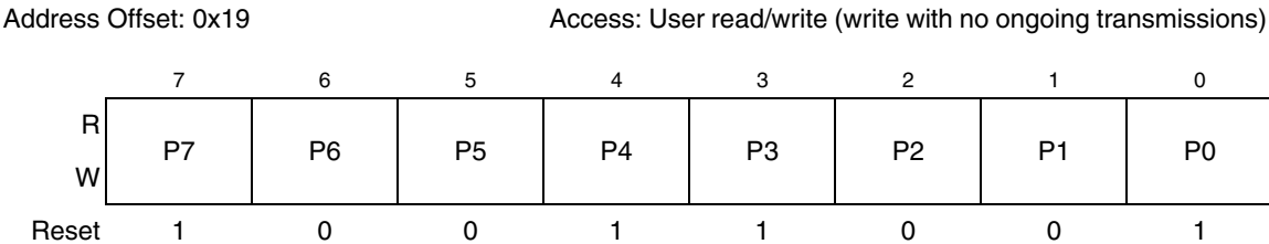
Figure 31-20. LIN CRC Polynomial Register 2 (LINCRCP2)
