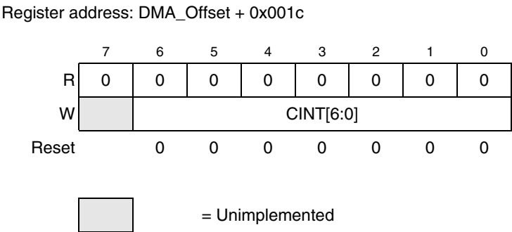
Figure 12-10. DMA Clear Interrupt Request (DMACINT) Register
