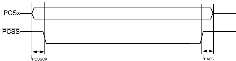
Figure 30-15. Peripheral Chip Select Strobe Timing
