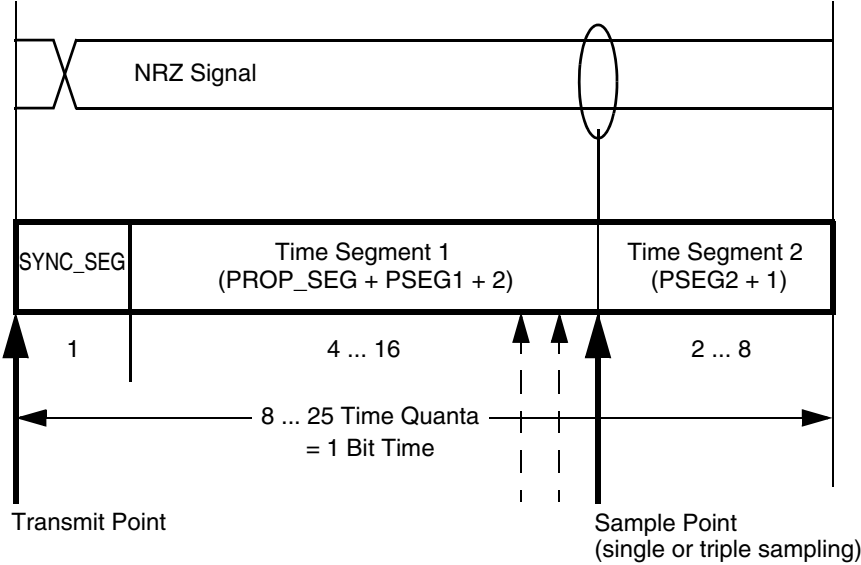
Figure 28-13. Segments within the Bit Time
