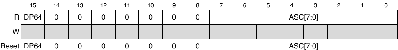
Figure 13-4. AXBS Slave Configuration (ASC) Register
