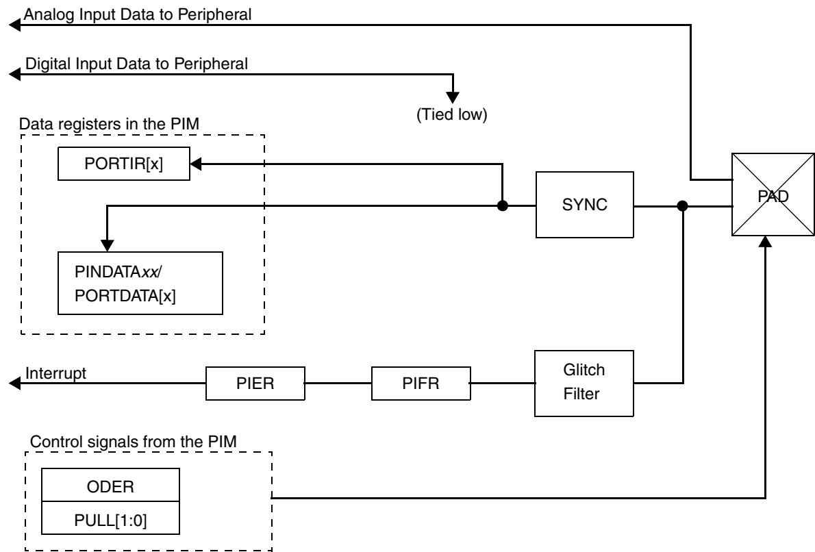
Figure 34-20. Pad in GPI Mode (including pad PD2)
