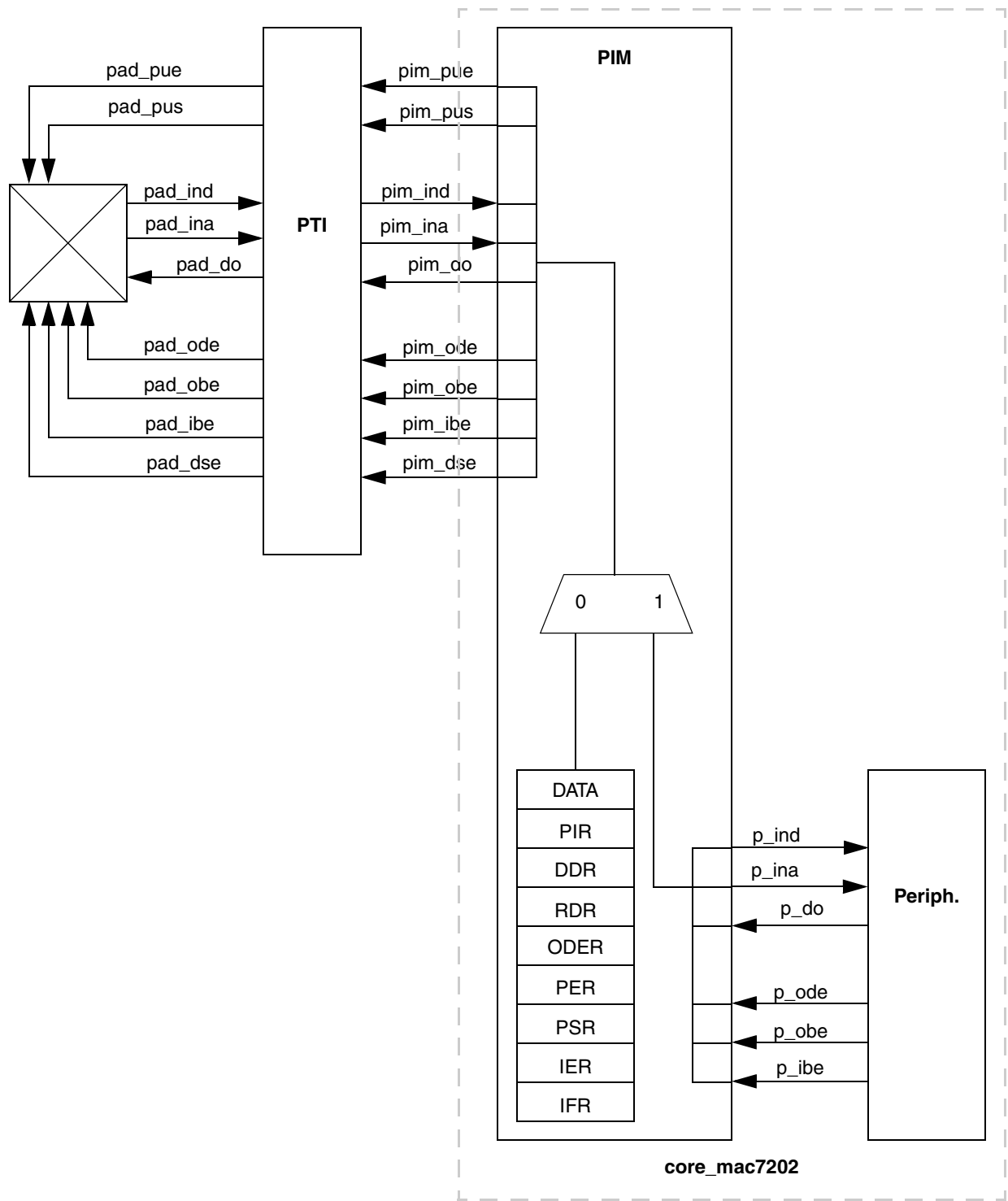
Figure 34-25. I/O Pad Control (Detailed View)
