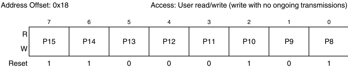
Figure 31-19. LIN CRC Polynomial Register 1 (LINCRCP1)
