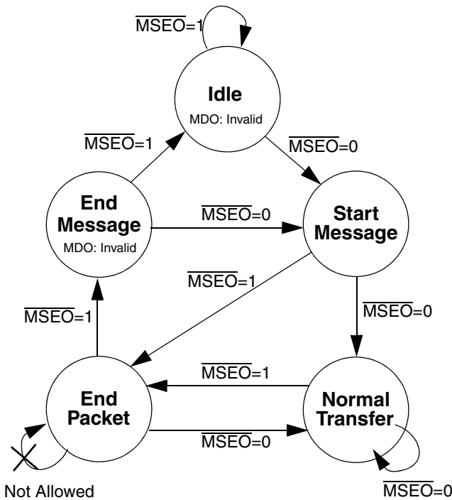
Figure 11-2. Single Pin \overline{\text{MSEO}} Transfers
