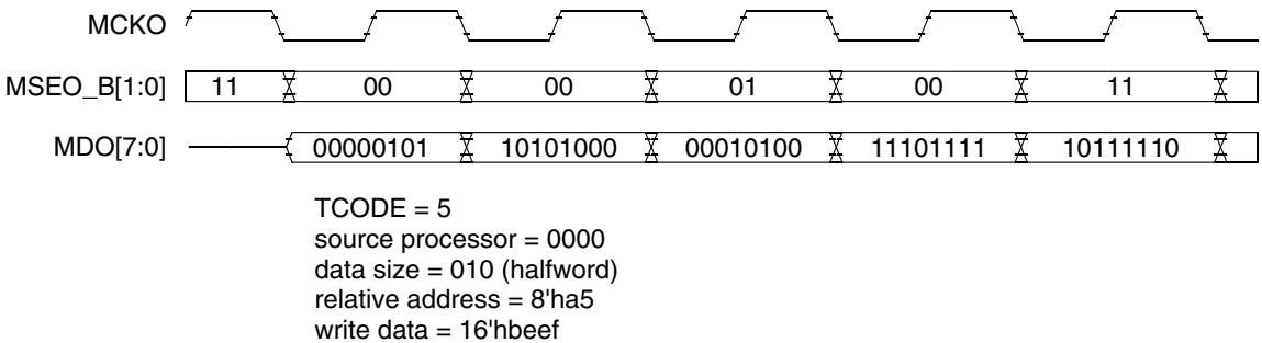
Figure 11-43. Data Trace – Data Write Message
