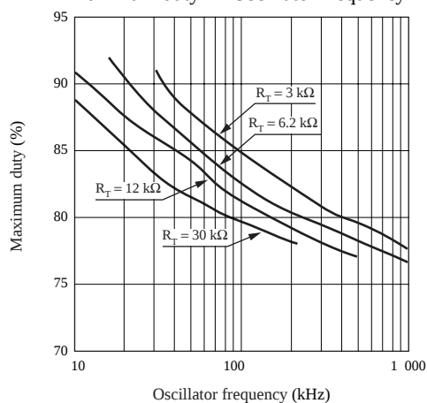
Maximum duty — Oscillator frequency
