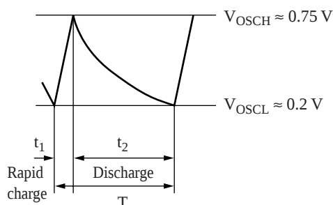
Figure 1. Triangular oscillator waveform
