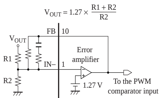
Figure 2. Connection method of error amplifier
