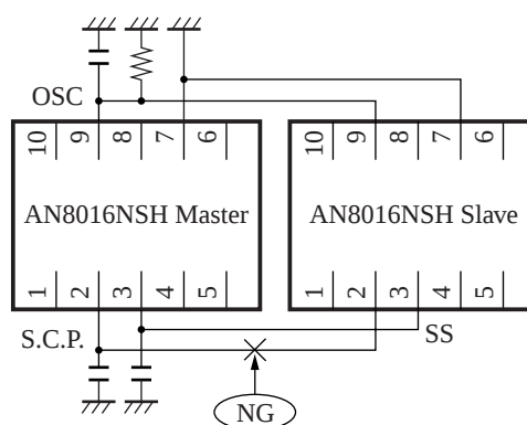
Figure 7. Slave operation circuit example
