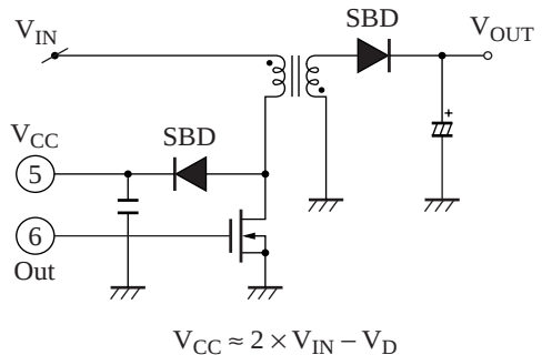
Figure 2. Gate drive voltage boosting technique
