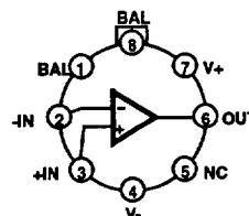
HA-5177 (TO-99 METAL CAN) TOP VIEW
