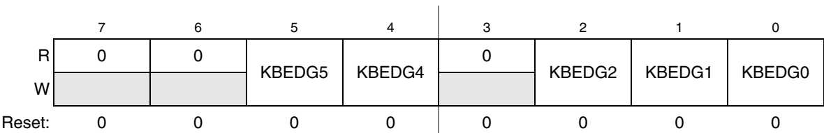
Figure 7-5. KBI Edge Select Register (KBIES)
