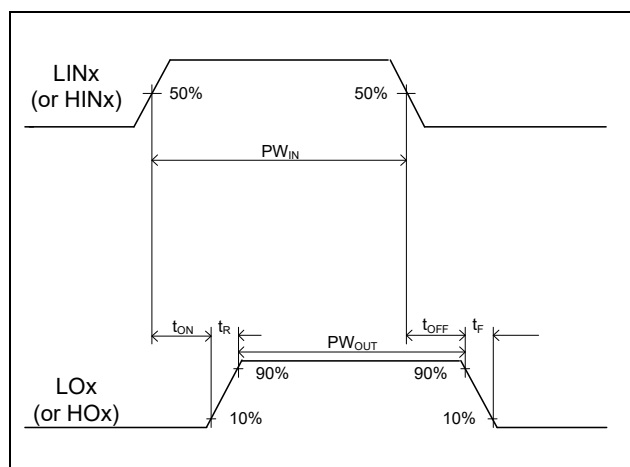
Figure 6 Switching timing diagram
