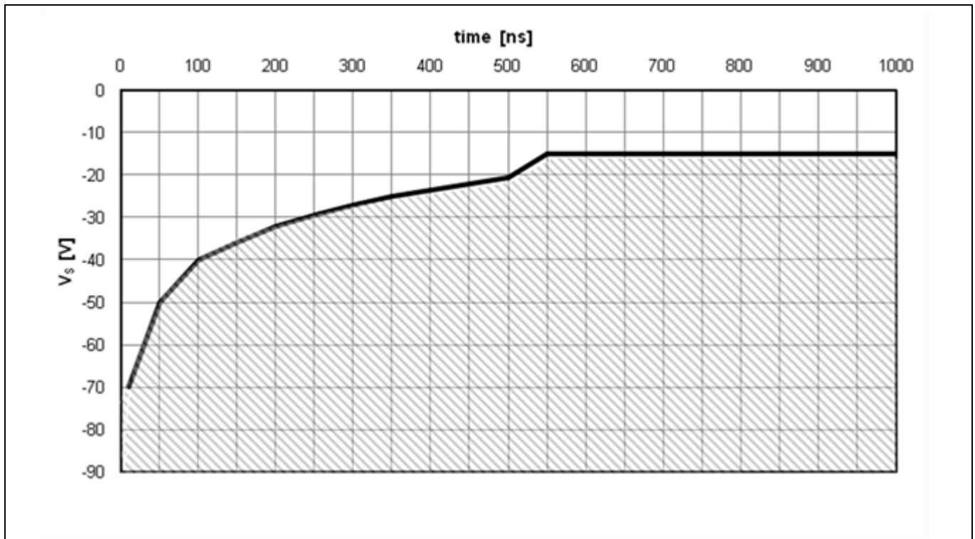
Figure 22 Negative V_S transient SOA for 2ED28073J06F @ V_{BS}=15\text{ V}
