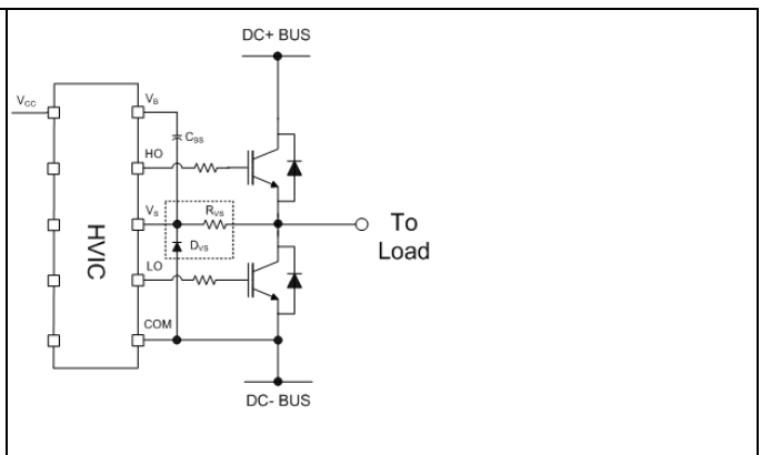
Figure 25 Clamping diode between COM and V_S
