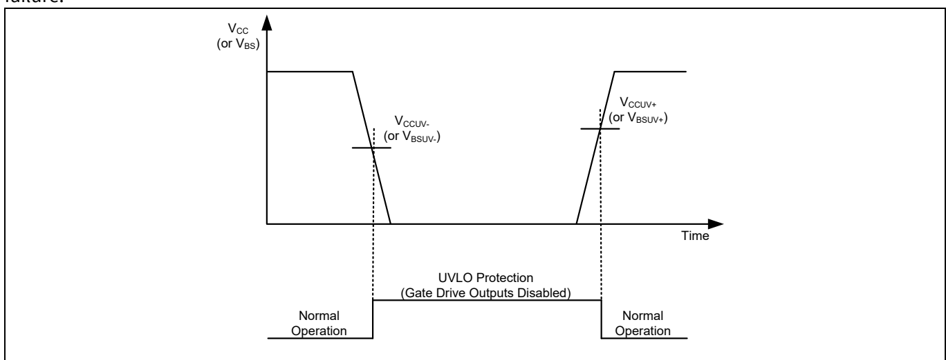
Figure 10 UVLO protection
