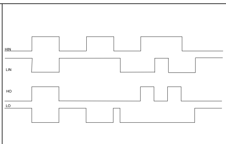
Figure 7 Input/output logic diagram
