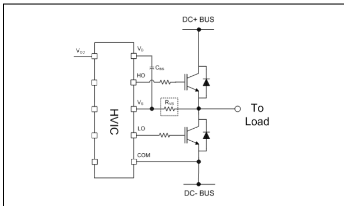
Figure 24 Resistor between the V_S pin and the switch node
