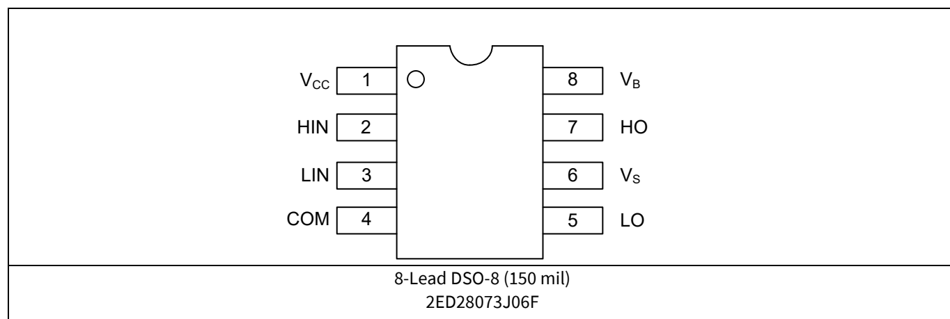
Figure 3 2ED28073JS06F pin assignments (top view)
