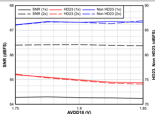
Figure 6-36. AC Performance vs AVDD18
