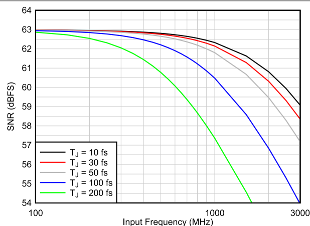
Figure 8-2. SNR vs T_{\text{Jitter}} vs F_{\text{IN}} (1x AVG)
