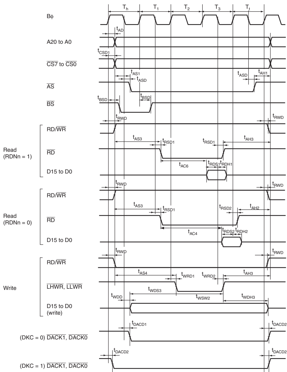
Figure 26.13 Basic Bus Timing: 3-State Access ( \overline{\text{CS}} Assertion Period Extended)
