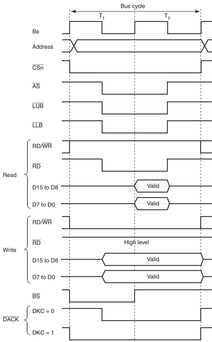
Figure 8.27 \overline{\text{DACK}} Signal Output Timing
