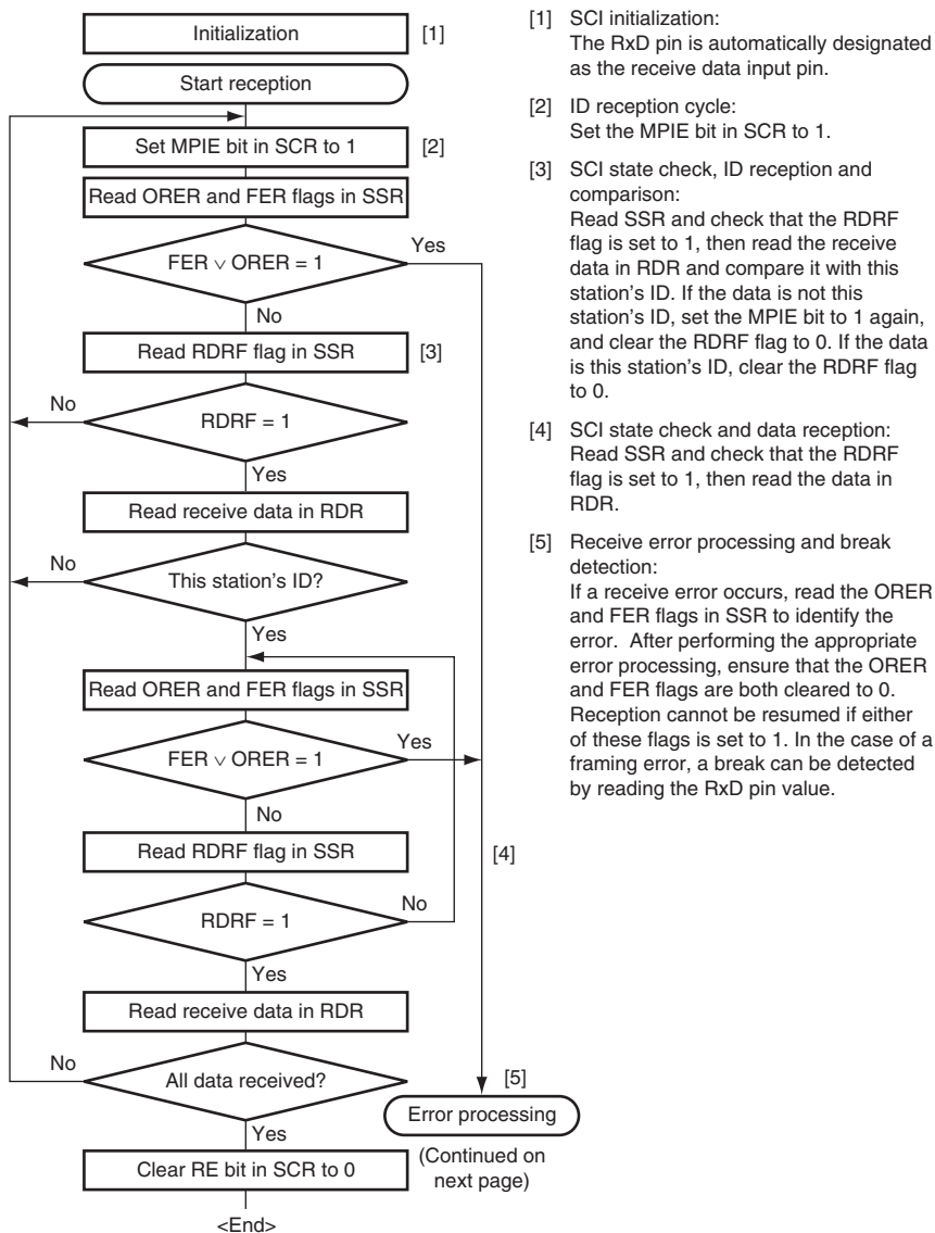
Figure 16.13 Sample Multiprocessor Serial Reception Flowchart (1)
