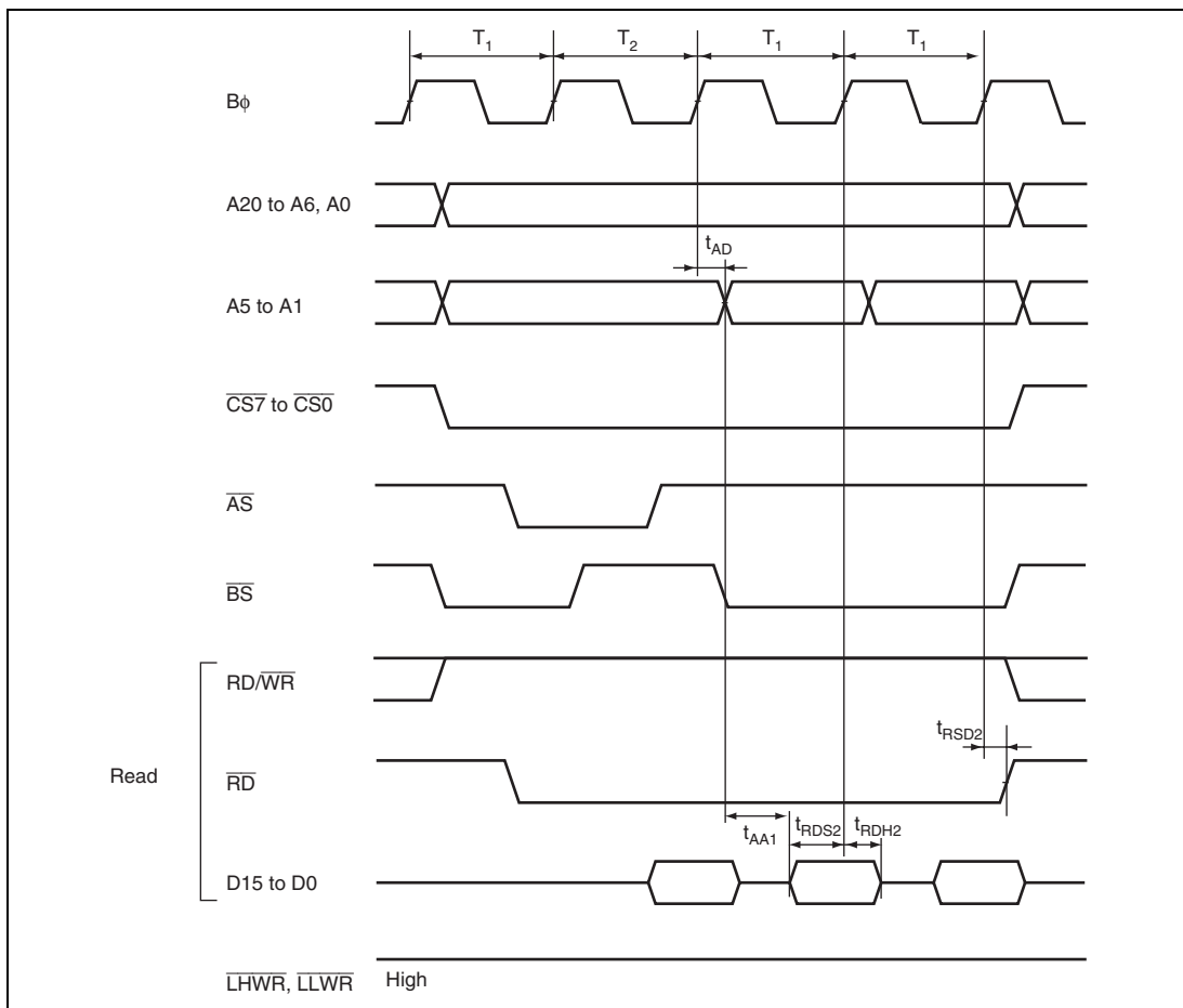
Figure 26.16 Burst ROM Access Timing: 1-State Burst Access
