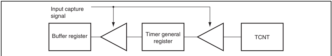
Figure 12.13 Input Capture Buffer Operation
