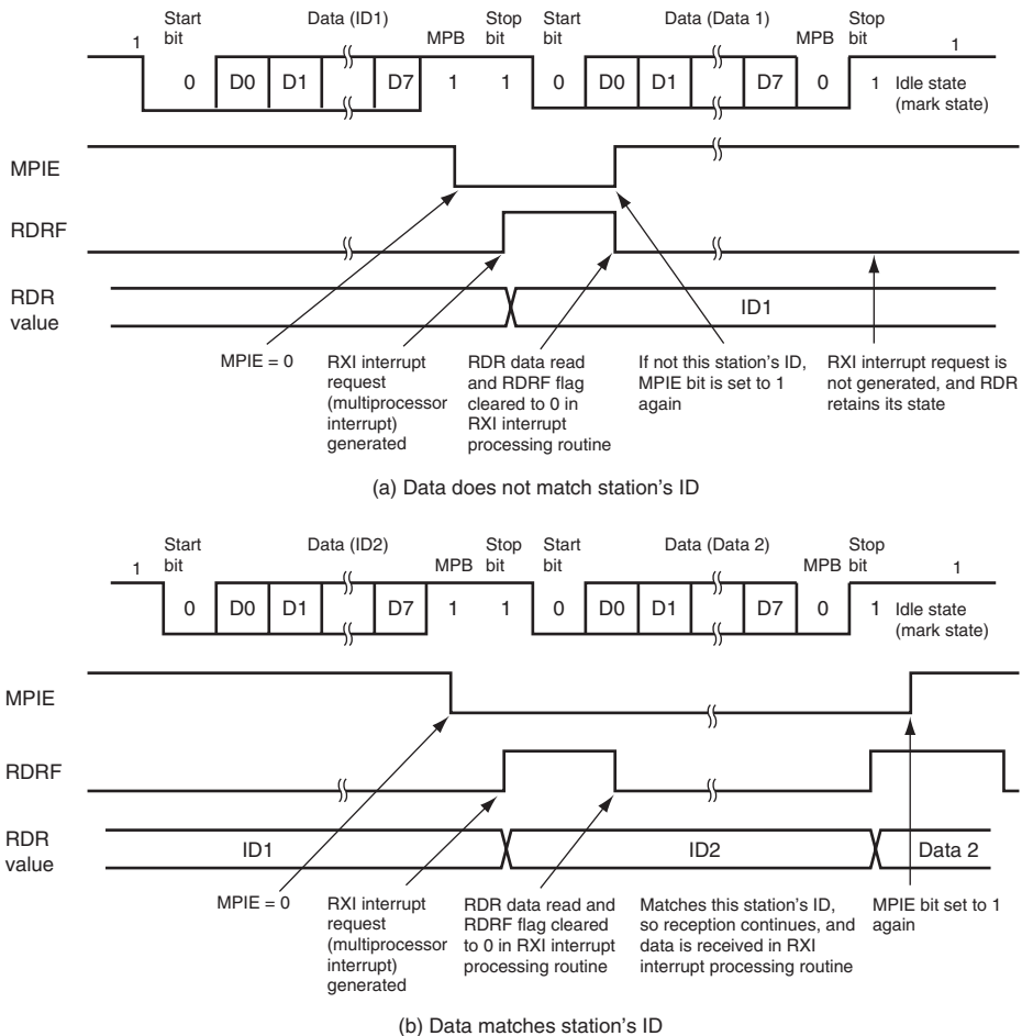
Figure 16.12 Example of SCI Operation for Reception (Example with 8-Bit Data, Multiprocessor Bit, One Stop Bit)
