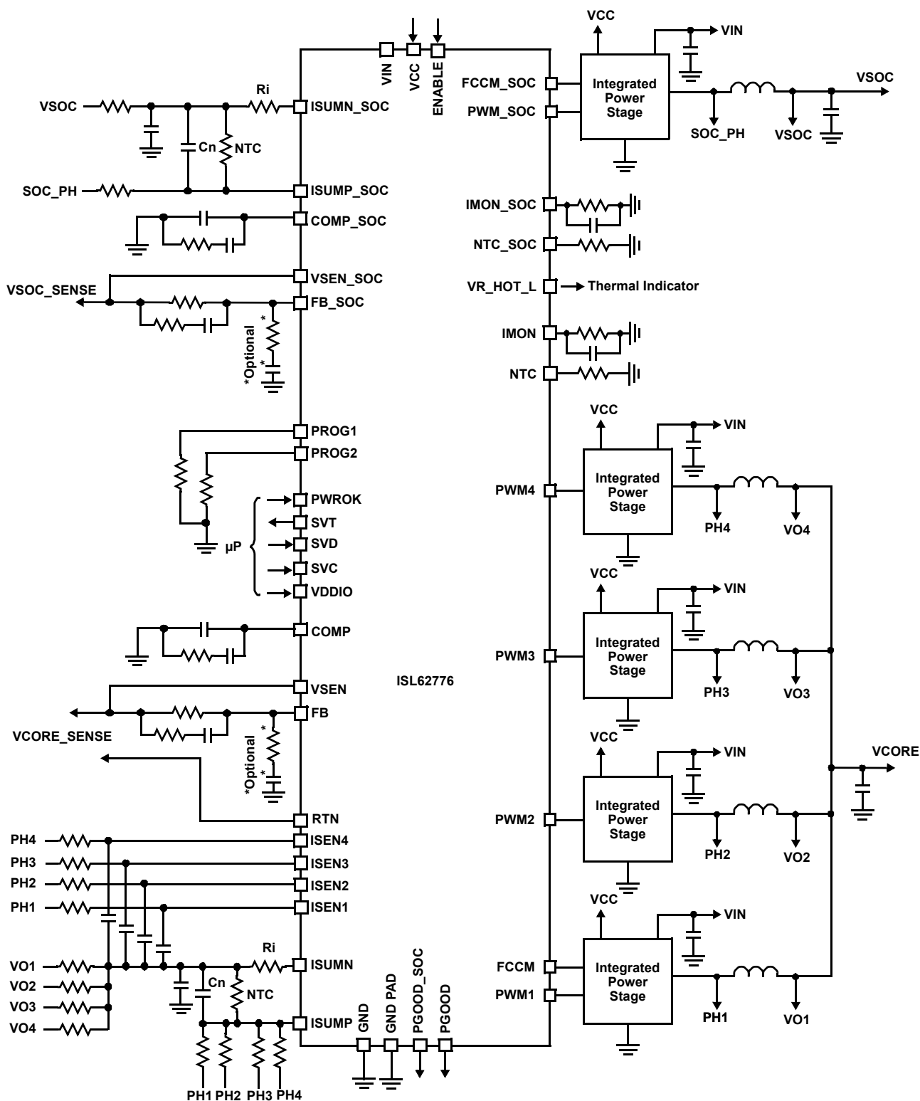
Figure 2. Typical Application Circuit for High-Power CPU Core Using Inductor DCR Sensing, 4+1
