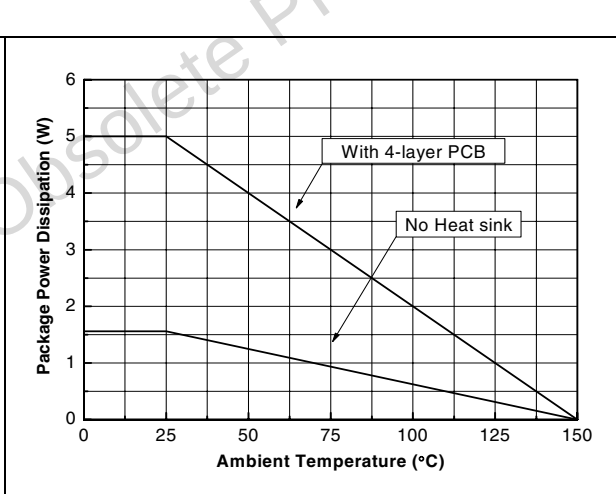
Figure 5. Power derating curves
