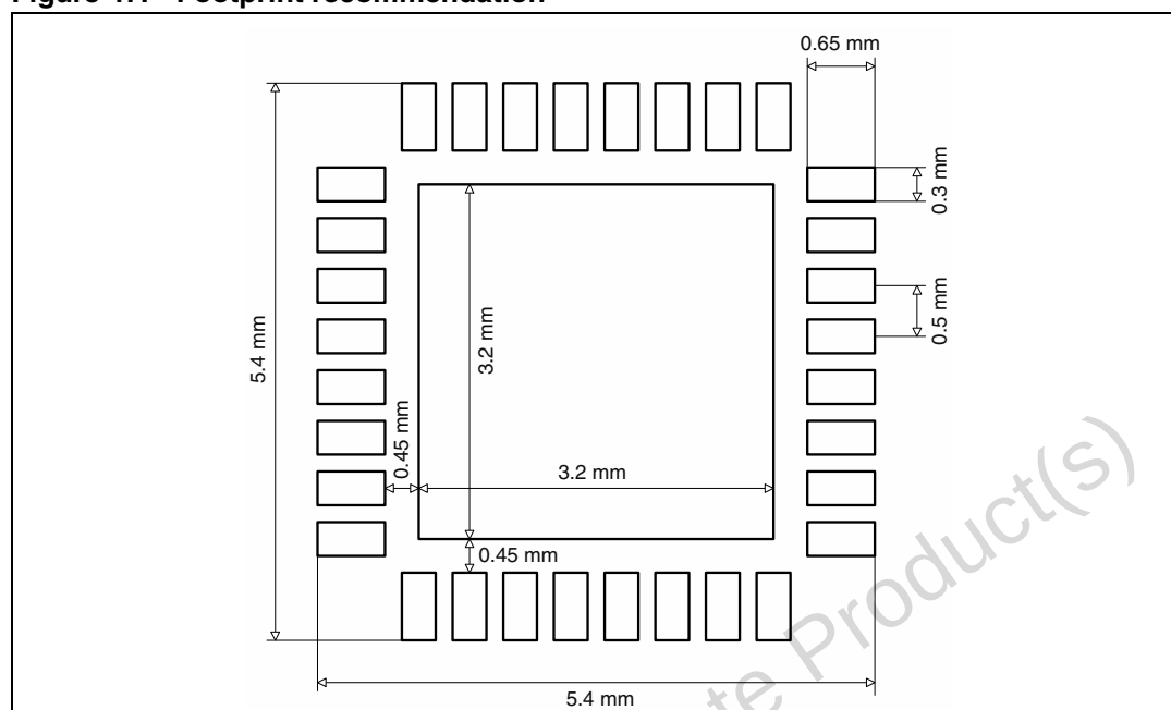
Figure 47. Footprint recommendation
