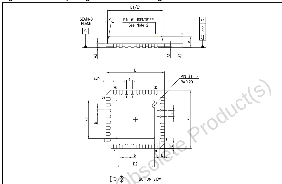
Figure 46. QFN32 package mechanical drawing
