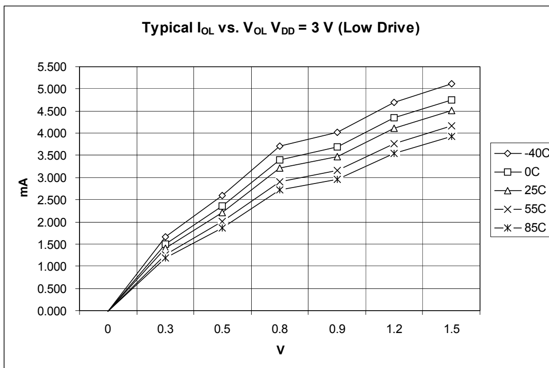
Figure 13. Typical I_{OL} Vs. V_{OL} ( V_{DD} = 3.0\text{ V} ) (Low Drive)
