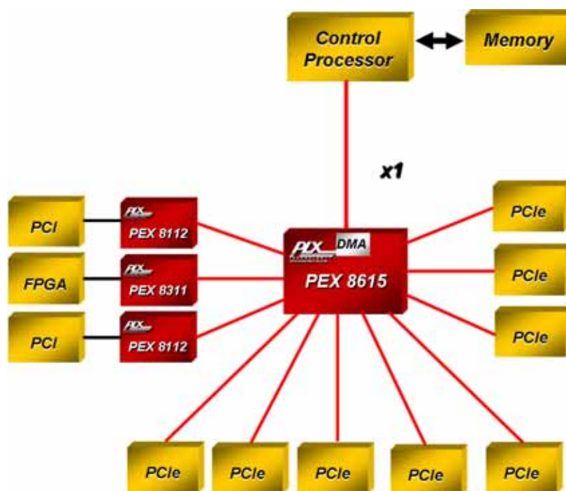
Figure 2-2. Fan-In/Fan-Out Usage
