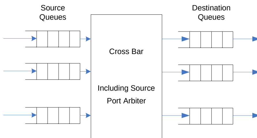
Figure 9-4. On-Chip Queuing
