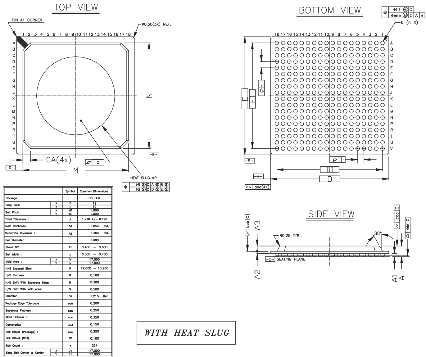
Figure 22-1. Mechanical Dimensions (19 x 19 mm 2 HSBGA Package)
