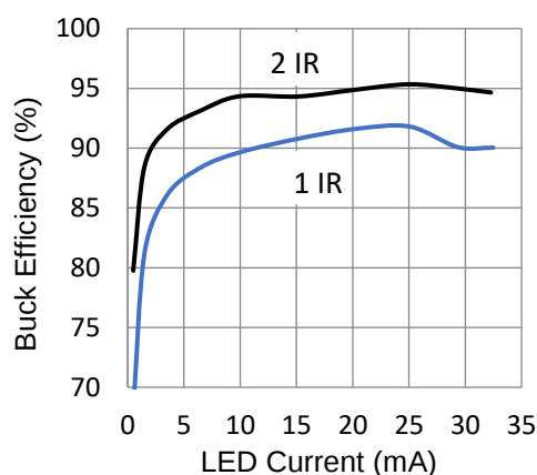
Buck Efficiency v. ILED (9 channels, Skip-mode, V_{IN} = 3.6V )
