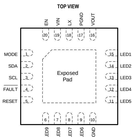
UQFN33-20
