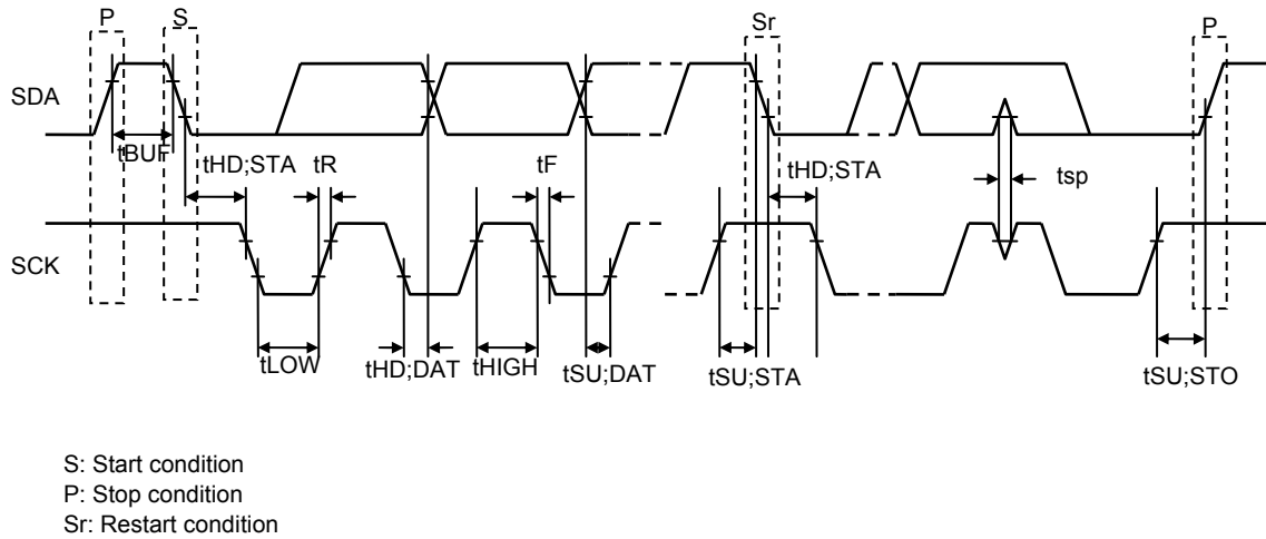
Figure 8 I²C Timing
