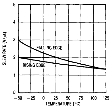
Slew Rate
