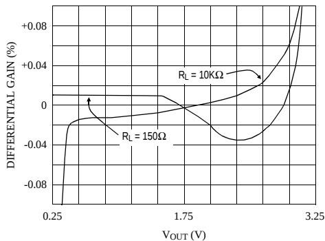
Differential Gain for R_L Tied to 2.5V
