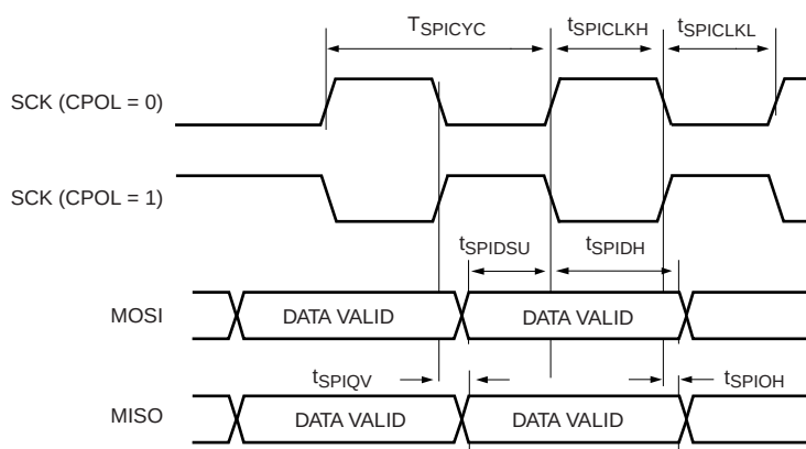
Fig 22. SPI slave timing (CPHA = 0)
