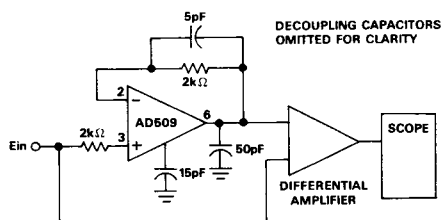
Figure 2. AD509 Settling Time Test Circuit
