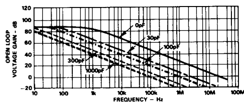
Figure 7. Open Loop Frequency Response for Various C_L 's
