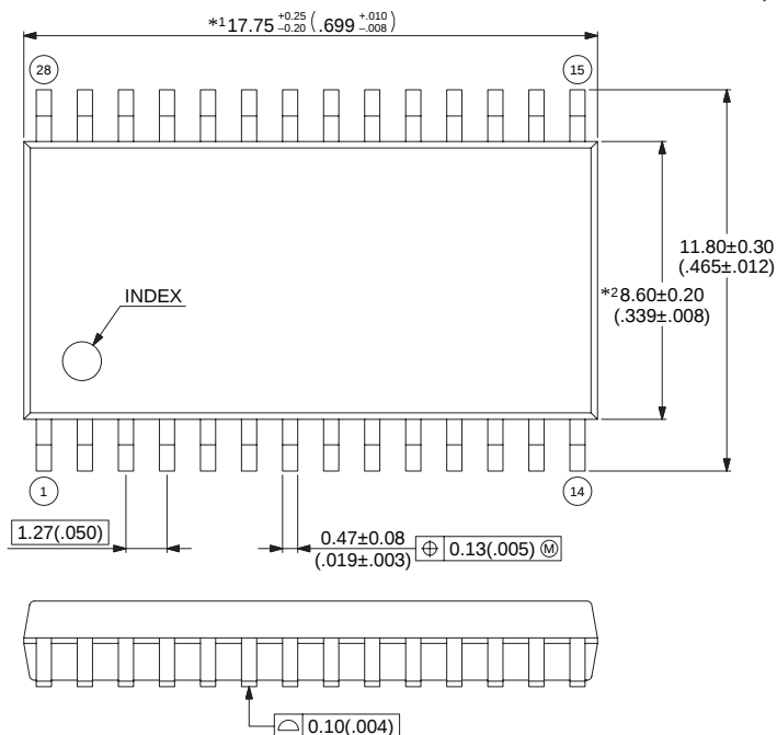
28-pin plastic SOP (FPT-28P-M17)
