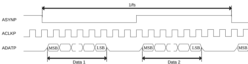
Fig23-5 RM_SYNC=0, PB_MASTER=0, ADATPDLY=1
