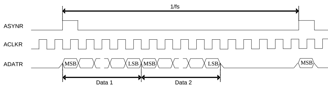
Fig23-4 RM_SYNC=1, PB_MASTER=0, ADATPDLY=1
