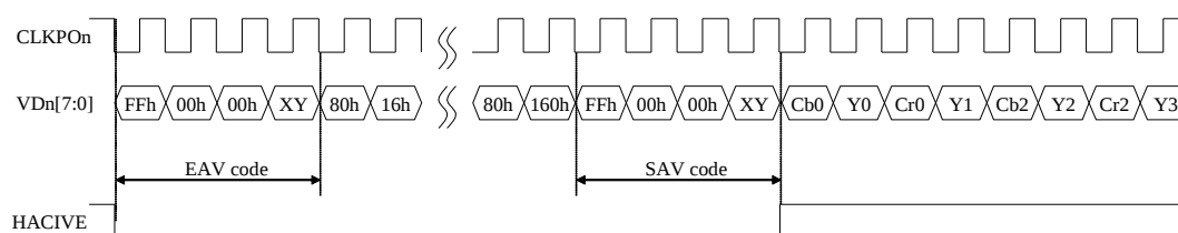
Fig9 Timing Diagram of ITU-R BT.656 format
