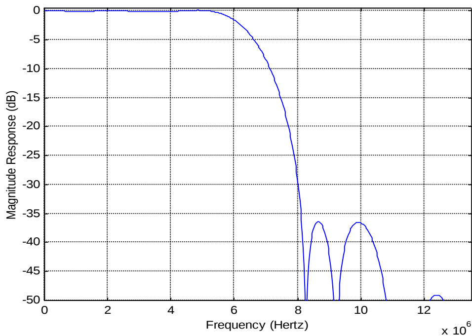
Fig2 The Characteristic of the Decimation Filter
