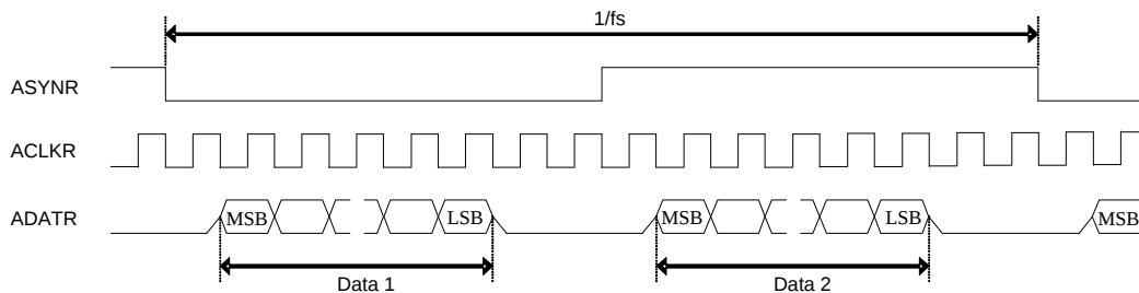
Fig22-1 ACLKMASTER=0, RM_SYNC=0
