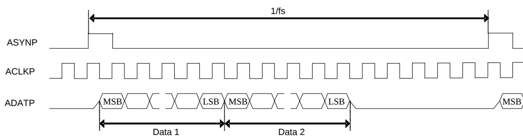
Fig23-6 RM_SYNC=1, PB_MASTER=0, ADATPDLY=1
