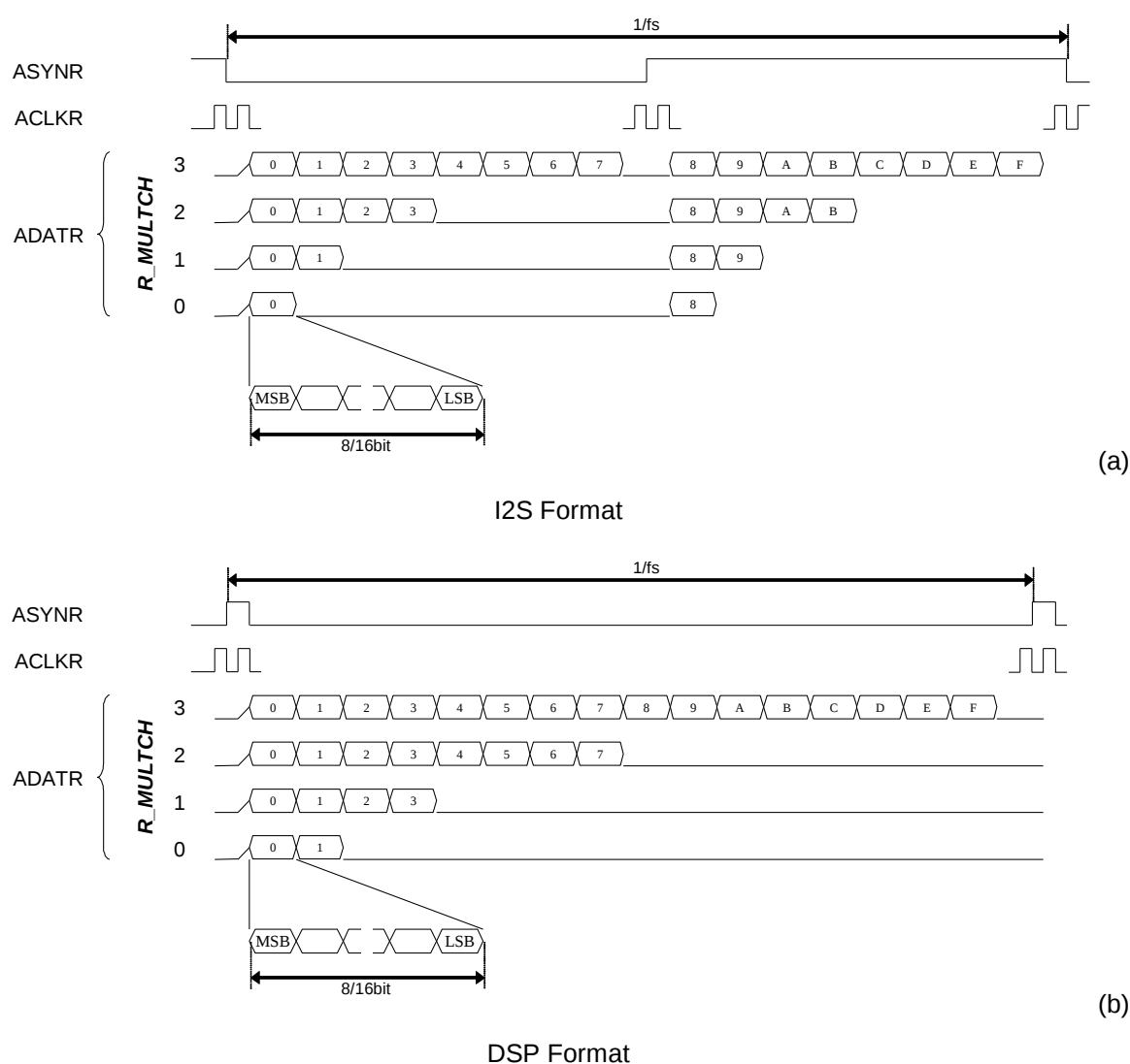
Fig21 Timing Chart of Multi-channel Audio Record
