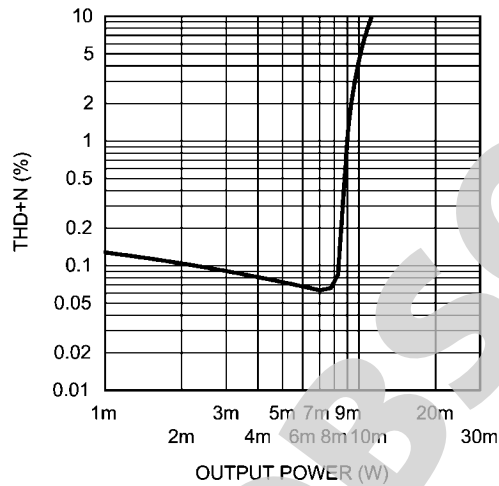
THD+N vs Output Power V_{DD} = 1.2V , R_L = 16\Omega , f = 1kHz A_V = -1 , Single Ended Output
