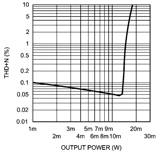
THD+N vs Output Power V_{DD} = 1.5V , R_L = 16\Omega , f = 1kHz A_V = -1 , Single Ended Output
