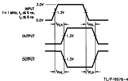
FIGURE 2. Propagation Delays
