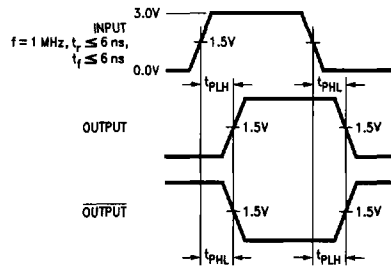
FIGURE 8. Load Propagation Delays for "LS-Type" Load
