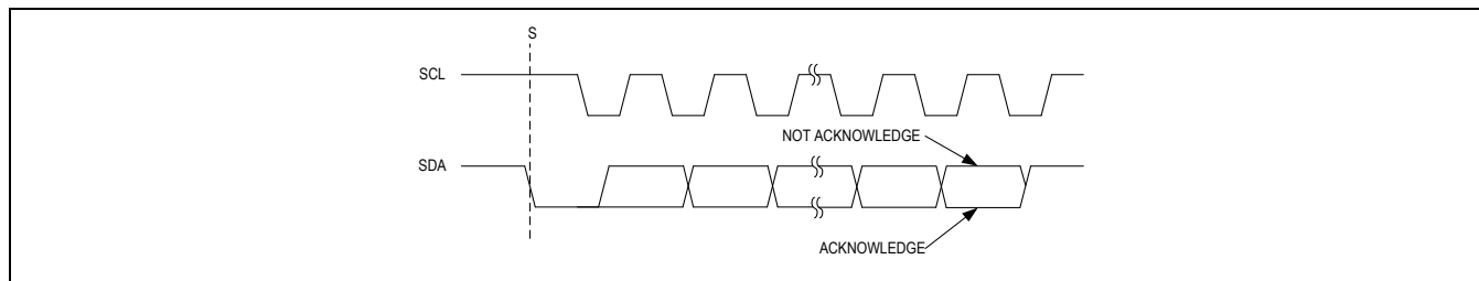
Figure 10. Acknowledge Bits
