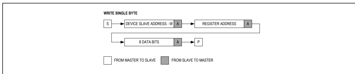
Figure 6. Write Byte Sequence
