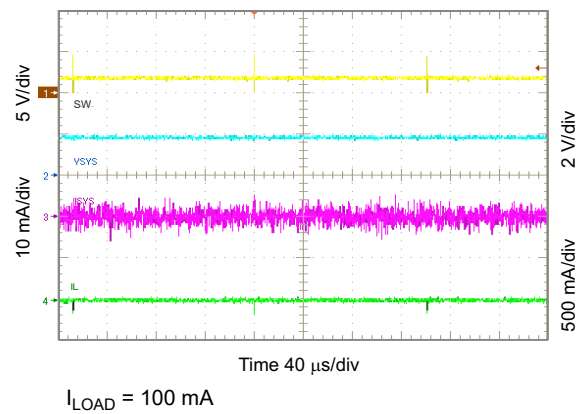
Figure 10-27. Light Load Operation Showing SW
