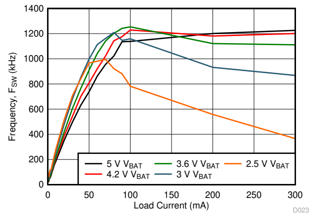
Figure 10-25. 1.8 V_{\text{SYS}} Switching Frequency vs Load Current
