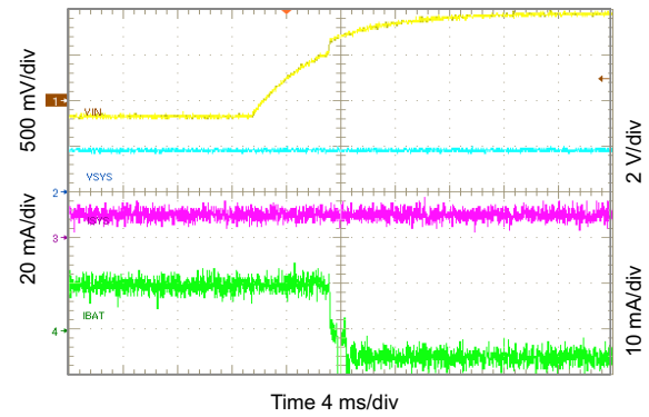
Figure 10-9. OVP Fault
