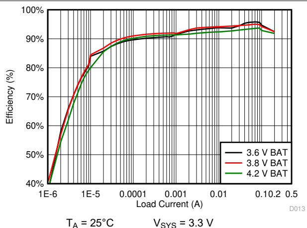
Figure 10-14. 3.3 V_{\text{SYS}} System Efficiency
