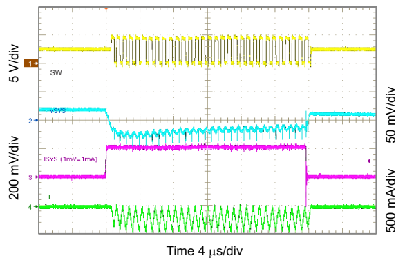
Figure 10-41. 2.5 V_{SYS} Load Transient, 0 to 200 mA
