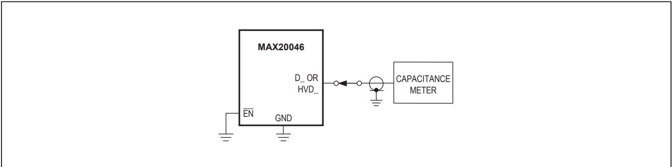
Figure 6. On-Capacitance
