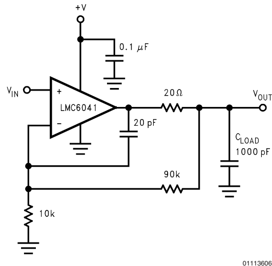
FIGURE 2. LMC6041 Noninverting Gain of 10 Amplifier, Compensated to Handle Capacitive Loads
