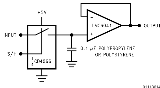
FIGURE 9. Low-Leakage Sample and Hold
