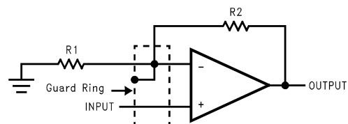
Non-Inverting Amplifier
