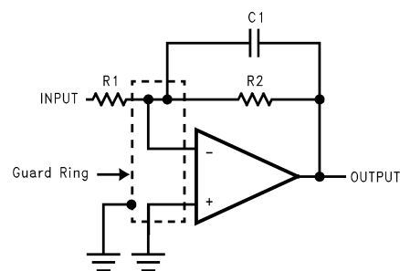
Inverting Amplifier
