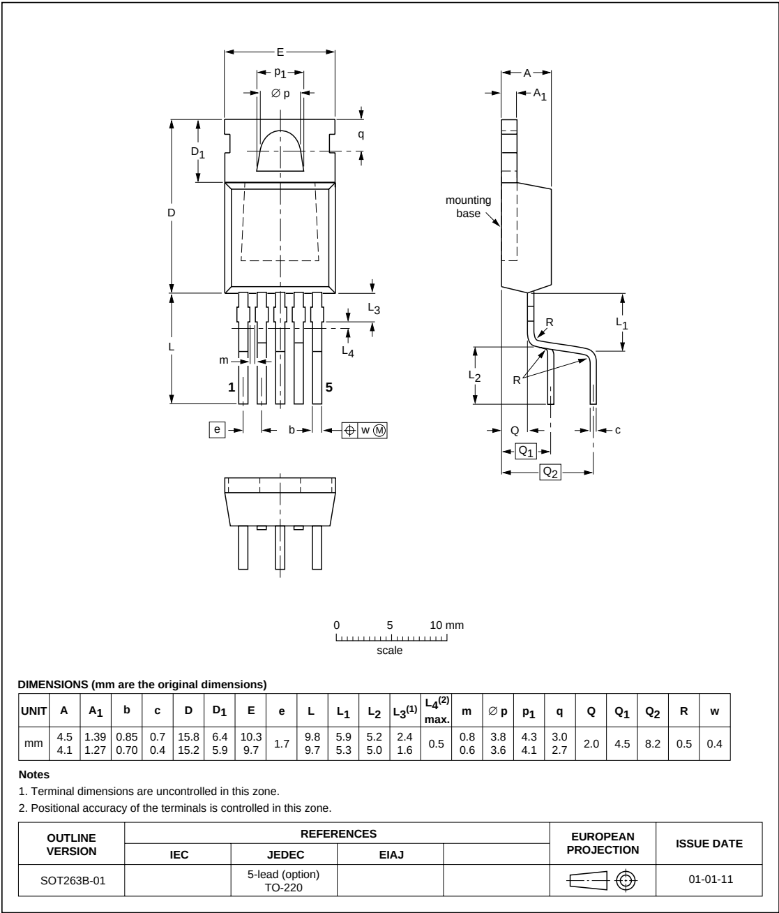
Fig.4. SOT263B package 1 leadform 263B-01, pin 3 connected to mounting base.
