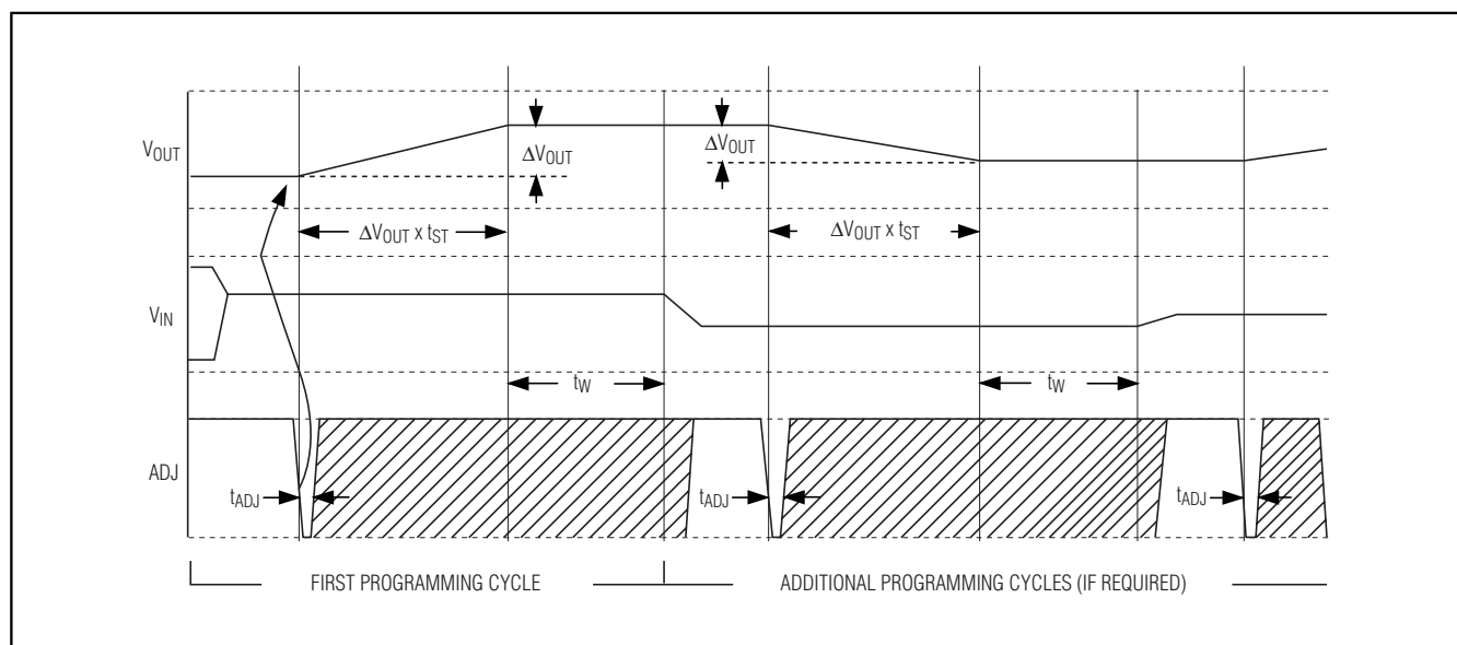
Figure 1. Timing Diagram
