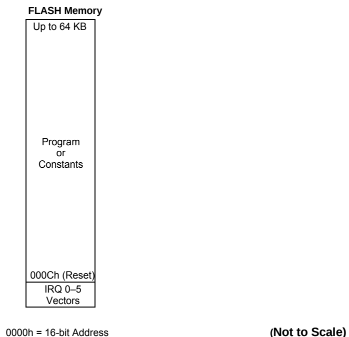
Figure 12. Program/Constant Memory Map
