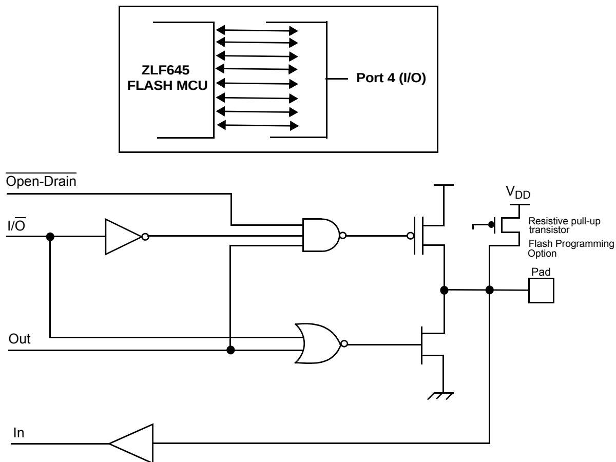
Figure 11. Port 4 Configuration
